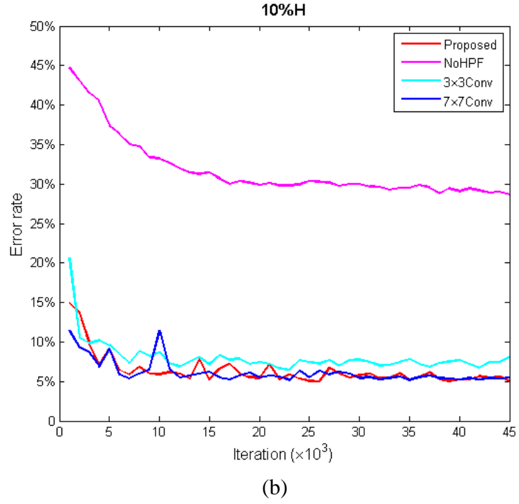
Figure 5.7 Training loss and testing error rate of four compared architectures on detecting horizontal seam carving with carving rate as 10%.
