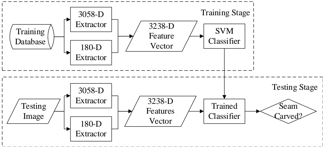
Figure 4.2 Framework of proposed 3238-D feature model.
