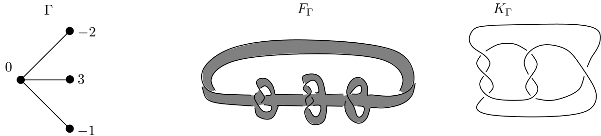
FIGURE 2. The plumbing graph \Gamma on the left determines a surface F_\Gamma (shown in the middle) with boundary K_\Gamma .
