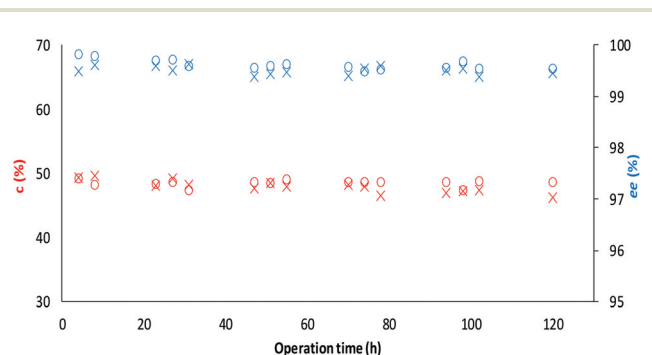
Fig. 8 Long term stability of the CaLB entrapped in the TDP sol-gel system in KR of the alcohol rac-1a ( c %: x, ee_{(R)-2a} : o) and amine rac-3a ( c %: o, ee_{(R)-4a} : x) in a continuous-flow reactor (60 °C, flow-rate of 0.1 mL min -1 ).
