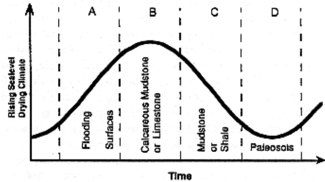
Figure 15. Illustration of climatic-eustatic model proposed here for the generation of meter-scale cycles within the Wolfcampian. The combined sea-level/climate curve is divided into four parts: (A) rising sea level and drying climate, (B) sea-level highstand and driest climate phase, (C) falling sea level and increasing rainfall, and (D) sea-level lowstand and wet climate phase. The times of carbonate and clastic deposition and nondepositional periods are indicated below the curve [based in part on Cecil's (1990) climate model]. This model explains the pervasive carbonate to clastic pattern of the cycles.
