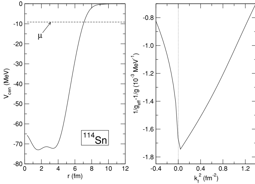
FIG. 5. The effective single-nucleon potential in ^{114}\text{Sn} as a function of the radial coordinate (left) and the correction to the strength parameter of the zero-range effective force as a function of the square of the Fermi momentum. \mu denotes the position of the chemical potential.
