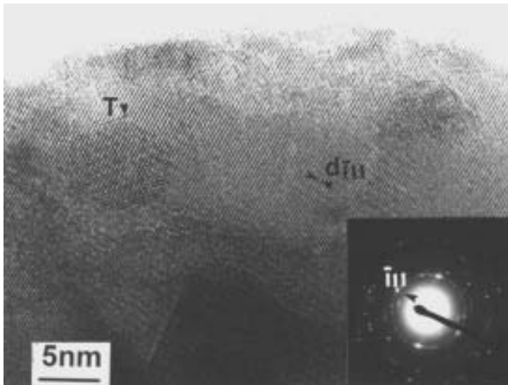
Figure 4. Nucleation of a small flake T of t\text{-ZrO}_2 on an m\text{-ZrO}_2 grain. The (\bar{1}11) lattice image, d = 0.316 nm. The corresponding ED pattern is given in the insert.
