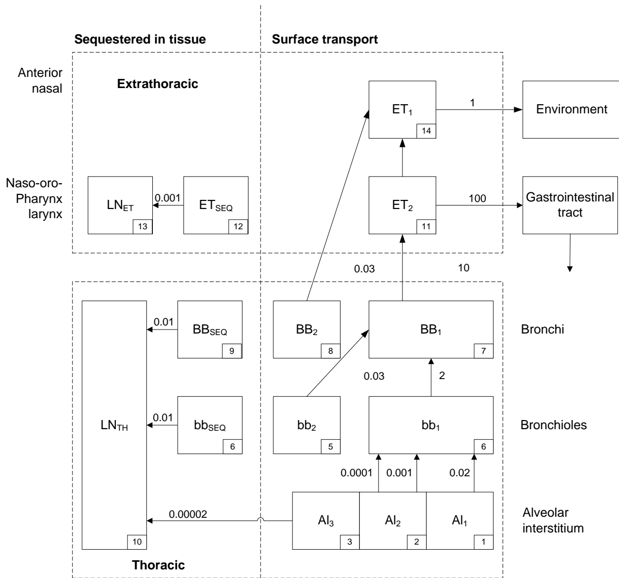
Figure 3-1. Respiratory Tract Compartments in Which Particles May be Deposited*
