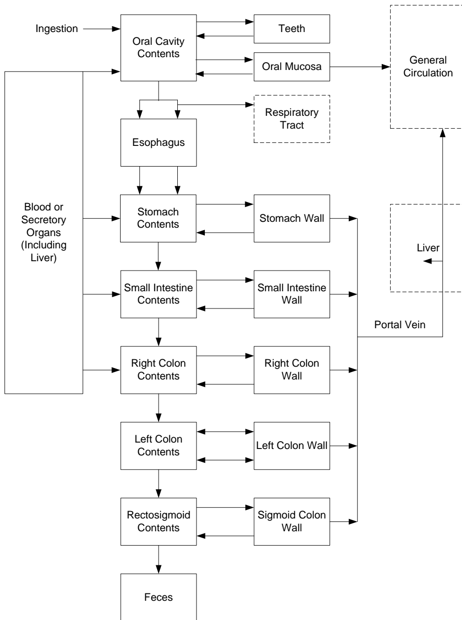
Figure 3-4. Structure of the Human Alimentary Tract Model (HATM)
