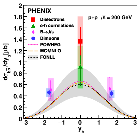
FIG. 27. Rapidity density d\sigma_{b\bar{b}}/dy_b in p+p collisions at \sqrt{s} = 200 \text{ GeV} measured in PHENIX via various channels compared to theoretical calculations. Here, y_b is the rapidity of a b quark.
