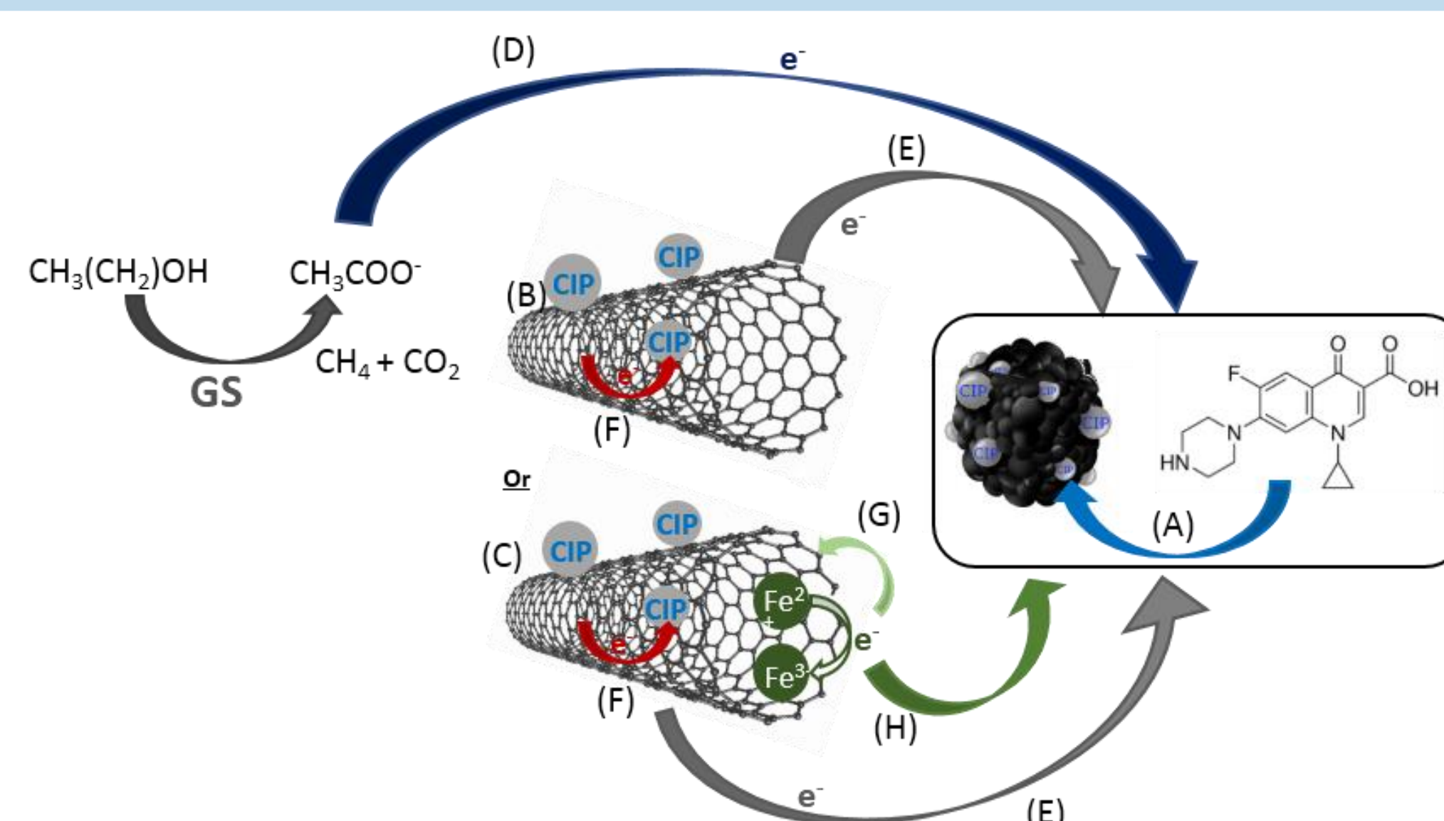
Figure 1 – Proposed mechanisms of CIP removal: adsorption on the sludge (A) ; adsorption on CNT (B) or CNT@2%Fe (C); electron (e - ) flow from the biological (GS) oxidation of ethanol to CIP (D) or to the CM and then to CIP, in solution or adsorbed on biomass (E) or adsorbed on the CM (F); e - transfer from the abiotic oxidation of Fe 2+ to CNT@2%Fe (G) and then to CIP (H) may also occur. All these mechanisms may occur independently or combined.
