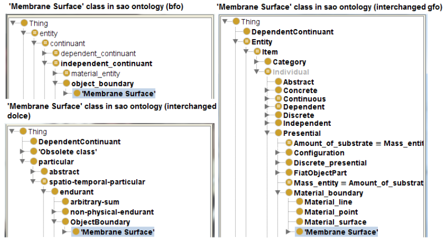
Fig. 1. The position of the sao:Membrane Surface class in source and target ontologies.
