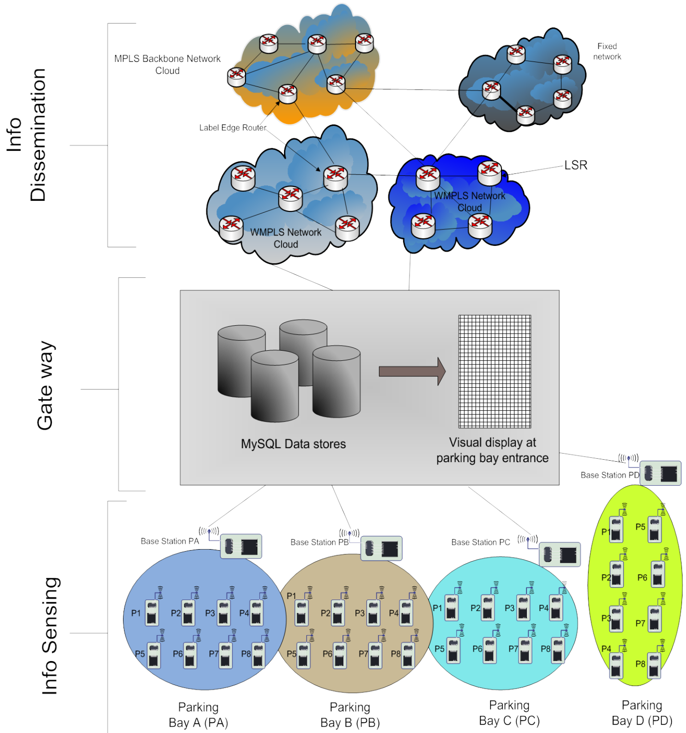
Figure 5: Architectural Design
