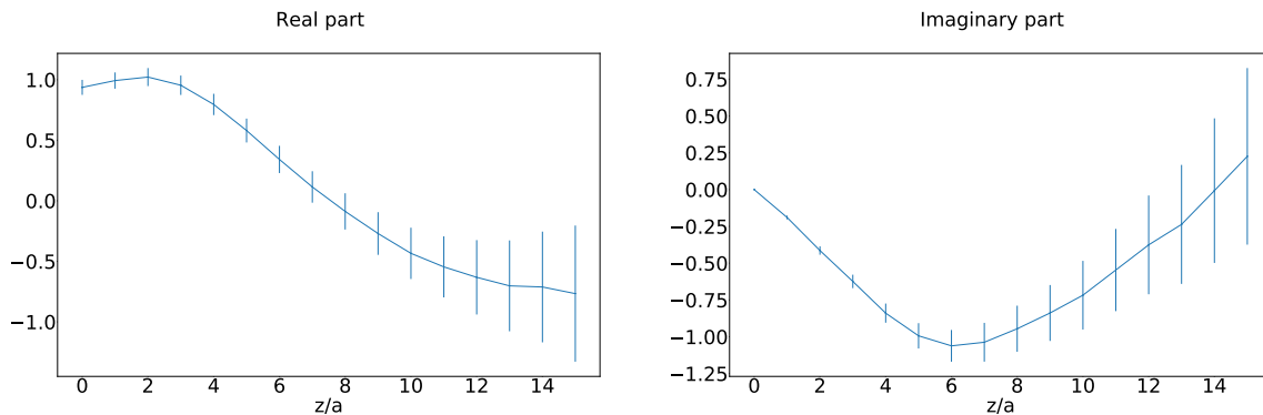
Figure 3.1. Real (left) and imaginary (right) part of the quasi-PDF ME for the data used in this work, computed in Refs. [30,45]. The error band displayed accounts only for statistical uncertainty. The separation z is expressed in units of the lattice spacing a .
