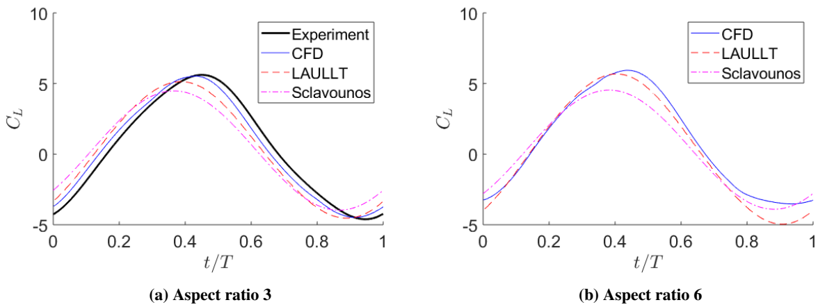
Fig. 20 C_L history for case 4: k = 1.0 , h_0/c = 0.5
