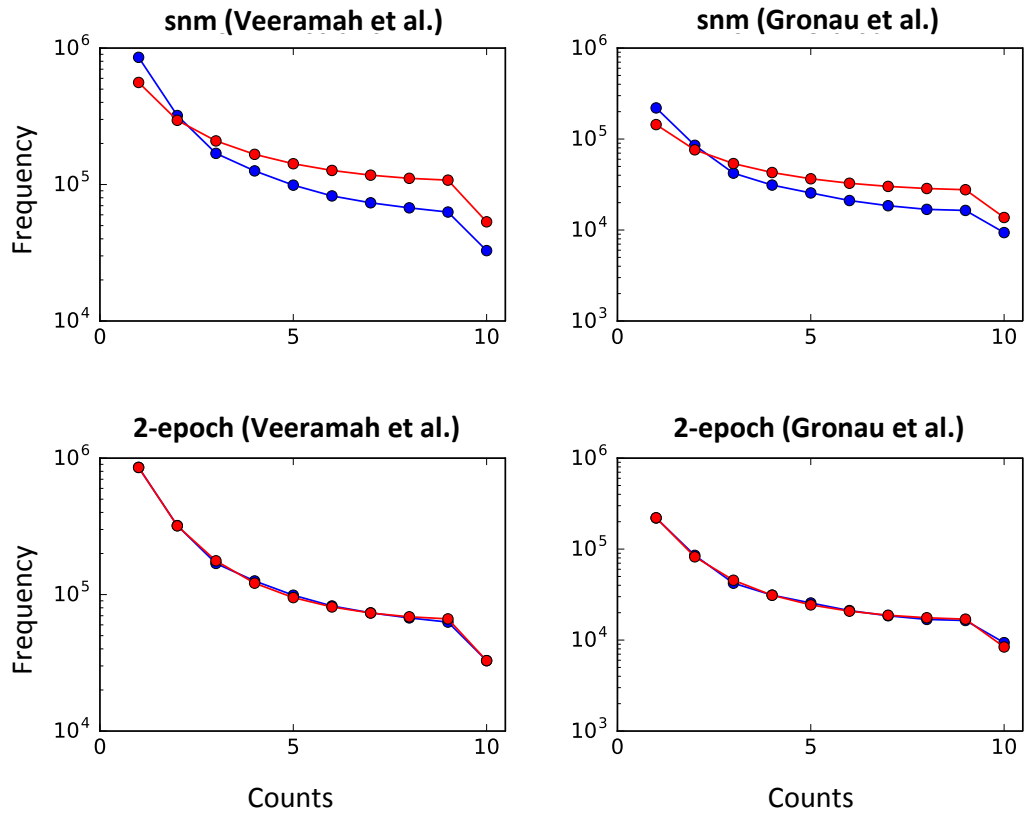
Figure S5. Comparison of standard neutral and best-fit 2-epoch models. Comparison of standard neutral model (snm) and best-fit 2 epoch model from \partial a \partial i against folded AFS based on non-genic loci from Veeramah et al. (18) and Gronau et al. (19).
