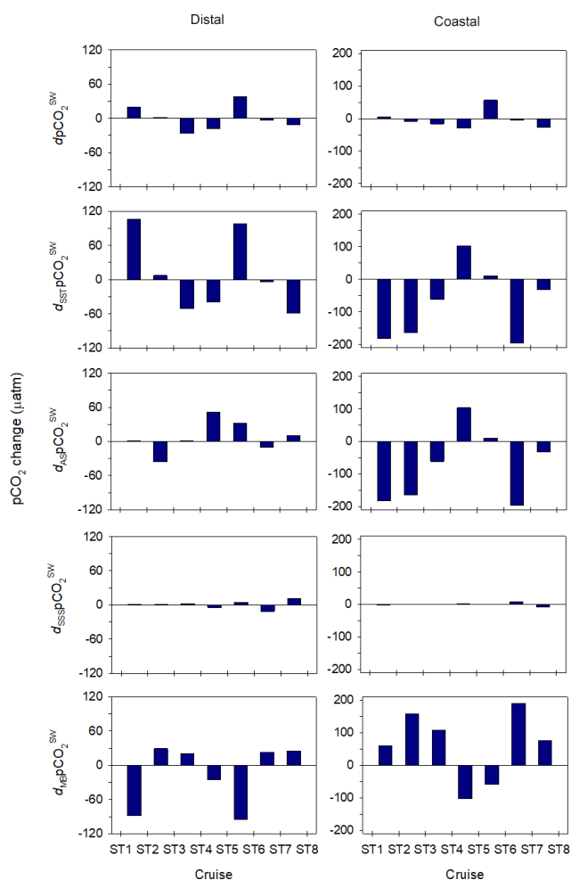
Figure 6. Observed changes in p\text{CO}_2 (first row) and p\text{CO}_2 changes broken down due to SST changes (second row), air–sea \text{CO}_2 exchange (third row), SSS changes (fourth row), and biology plus mixing (last row) in the distal (left column) and coastal areas (right column) between the periods of each cruise: ST1 (March 2014), ST2 (June 2014), ST3 (October 2014), ST4 (December 2014), ST5 (March 2015), ST6 (June 2015), ST7 (September 2015) and ST8 (February 2016).
