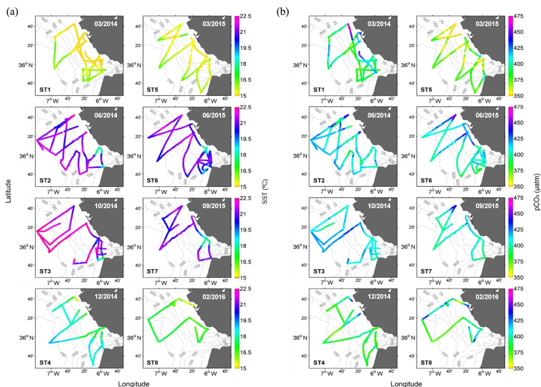
Figure 2. Underway distribution of sea surface temperature (SST ( ^{\circ}\text{C} ), a ) and p\text{CO}_2 ( \mu\text{atm} , b ) during the eight cruises in the Gulf of Cádiz: March 2014 (ST1), June 2014 (ST2), October 2014 (ST3), December 2014 (ST4), March 2015 (ST5), June 2015 (ST6), September 2015 (ST7) and February 2016 (ST8).
