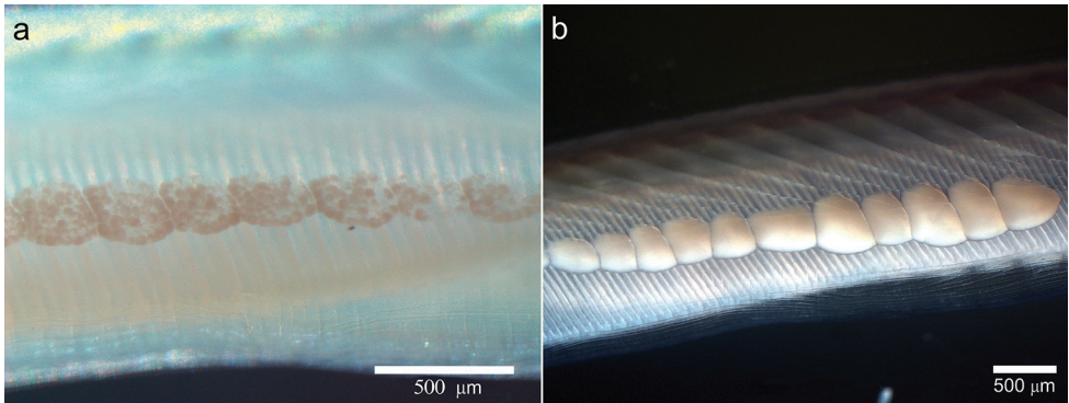
Figure 5. Sexual differentiation in amphioxus B. californiense , mature individuals: a female, with signs of some gonads having spawned (right side of the picture) b male with well-developed gonads (right side of the picture) and some gonads in the process of development (left side of the picture).
