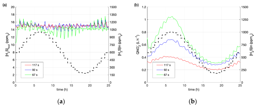
Figure 4. Profiles obtained in EBRT studies at 67 s, 92 s and 117 s. (a) H 2 S outlet concentration, (b) nitrite flowrate. Green lines: 67 s; blue lines: 92 s; red lines: 117 s; dashed black lines: H 2 S in .
