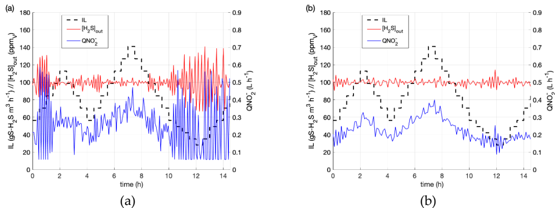
Figure 3. Staircase perturbation for PID (a) and PI (b) adjusted by MO. Blue lines: nitrite flowrate, red lines: H 2 S out , dashed black lines H 2 S IL.
