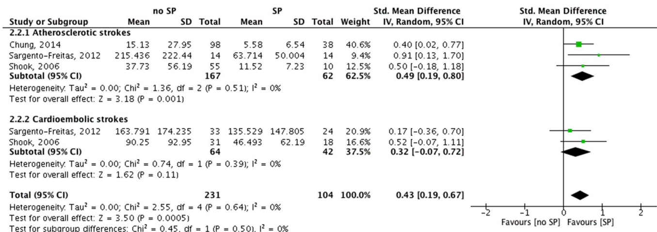
Fig. 2. Forest plots.
