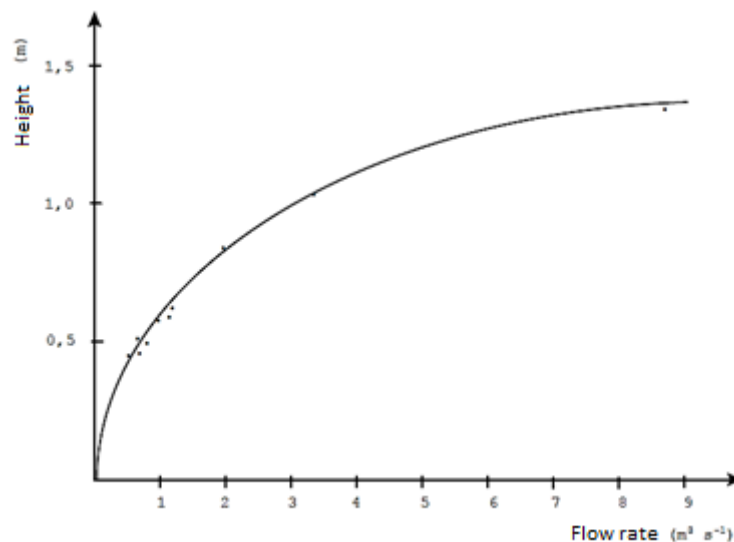
Figure 55 – Flow curve (Rodrigues et al., 2011).
