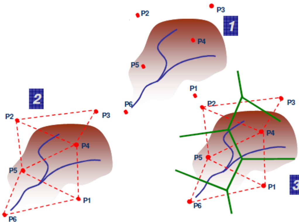
Figure 42 – Thiessen method (IST, 2018).
