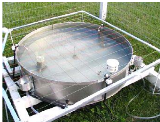
Figure 83 – Evaporimeter ( http://www.iginstrumentos.com.ar ).
