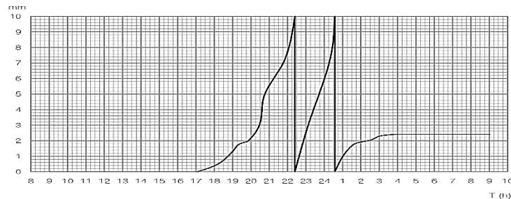
Figure 36 – Example of an udogram (Source: https://fenix.isa.ulisboa.pt/qubEdu/conteudos-publicos/ficheiros?oid=3972844804408 ).
