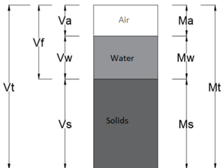
Figure 89 – Represent a column of soil with all agglutinated phases (adapted Hillel, 2004).
