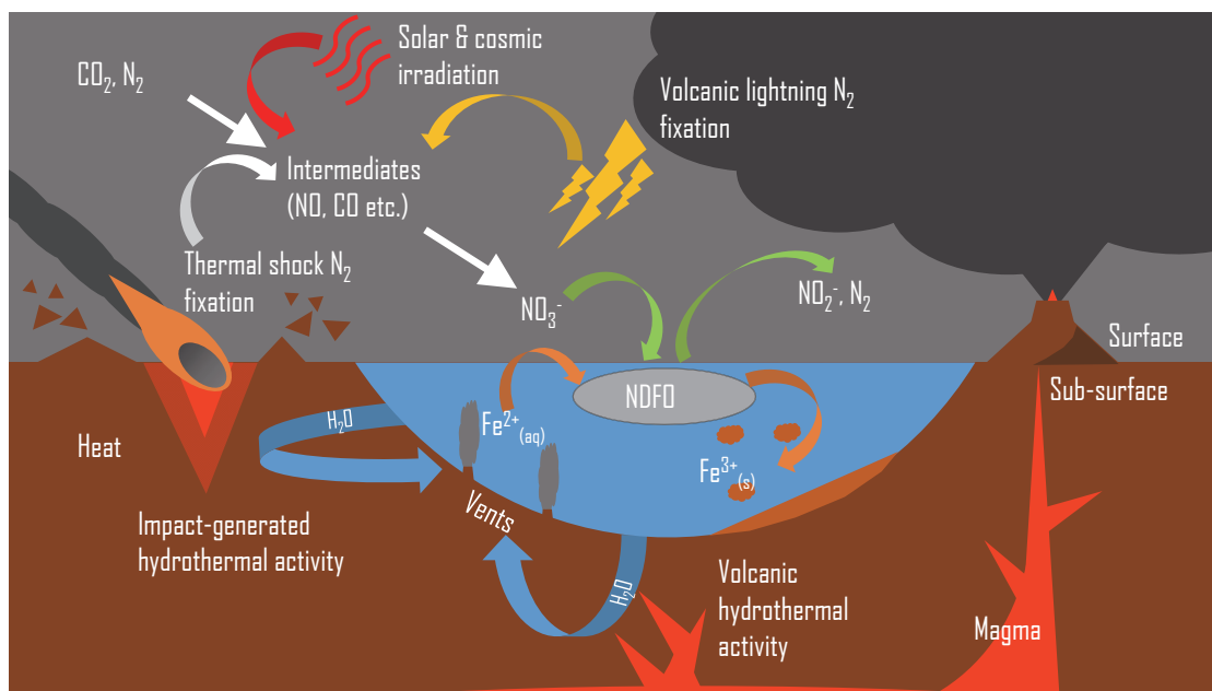
Figure 1. Potential energy sources and cycles for nitrate-dependent iron-oxidizing (NDFO) microbes on early Mars (Price, A., Pearson, V.K., Schwenger, S.P., Miot, J. and Olsson-Francis, K. (2018) Nitrate dependent iron oxidation: a potential Mars metabolism. Frontiers in Microbiology 9, 513)
