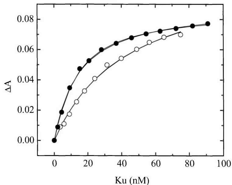
Figure 3-11 Binding isotherms for the s20 and s25 duplexes. The experiments were performed in buffer A at 300 mM NaCl and 25°C. The DNA concentration was 5 nM for the s20 (○) and 5 nM for the s25 (●). The same experiments were also repeated using a DNA concentration of 10 nM. For analysis of the binding curves, the free ligand concentration ( x_{\text{free}} ) was derived from equation 8. The fit of the data with equation 7 yielded k_d values of 77 \pm 7 nM (s20) and 29 \pm 2 nM (s25). The same analysis performed assuming x_{\text{free}} = x_T produced binding curves that are basically superimposable to the previous ones.
