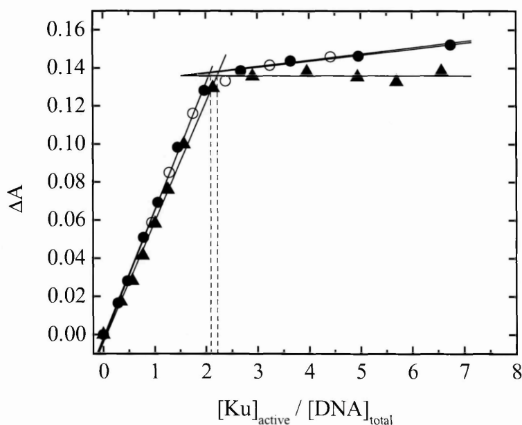
Figure 3-7 Stoichiometry determination for the s42 and s50 duplexes. Plot of the anisotropy changes vs. the ratio of active Ku over total DNA concentration. The duplexes used were: s50, 5 nM ( \blacktriangle ); s42, 5 nM ( \circ ); s42, 10 nM ( \bullet ). The experiments were carried out under saturating conditions \text{DNA}_{\text{total}} \gg k_d ( <0.2 nM) in buffer A at 100 mM KCl and 25°C. The stoichiometry was calculated from the crossing point of the two straight lines.
