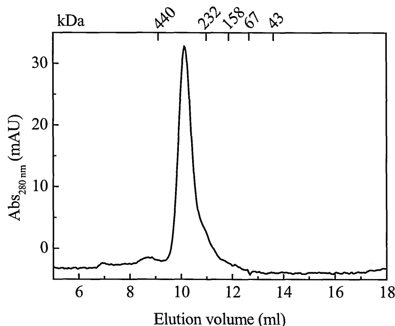
Figure 3-2 Gel filtration analysis of rKu70/80. \sim 200 \mu\text{g} of rKu70/80 were analysed using Superdex 200 HR 10/30 column. The numbers on the top indicate the molecular mass of protein standards.
