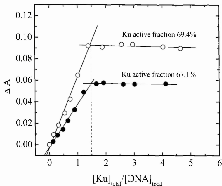
Figure 3-6 Determination of the active fraction of rKu70/80. Plot of the anisotropy changes \Delta A vs. the ratio [\text{Ku}]_{\text{total}}/[\text{DNA}]_{\text{total}} . \Delta A = A_{\text{obs}} - A_0 , where A_{\text{obs}} is the experimentally observed anisotropy signal and A_0 is the initial anisotropy signal. Data obtained respectively with the 20 (○) and 25 (●) bp duplexes (s20 and s25). Both DNA molecules were at a concentration of 5 nM ( \gg k_d ). The experiments were performed in buffer A at 100 mM KCl and the temperature was set at 25°C. Solid lines are the linear fit of proper portion of the dataset. The active fraction is derived from the value of the crossing point of the two straight lines ( 1/1.490 = 0.671 \times 100 = 67.1\% ).
