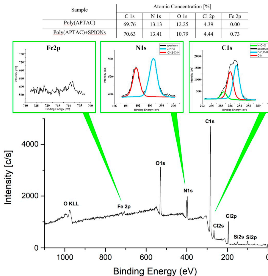
Figure 6. X-ray photoelectron spectroscopy (XPS) spectrum of poly(APTAC)+SPIONs with fragments corresponding to binding energies for Fe2p, N1s and C1s.
