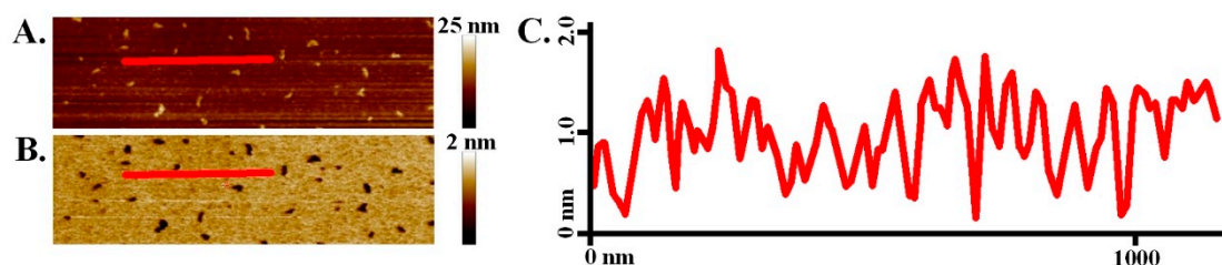
Figure 4. Poly(APTAC)+SPIONs brushes AFM images: topography (A) and indentation (B) with corresponding indentation image cross-section (C).
