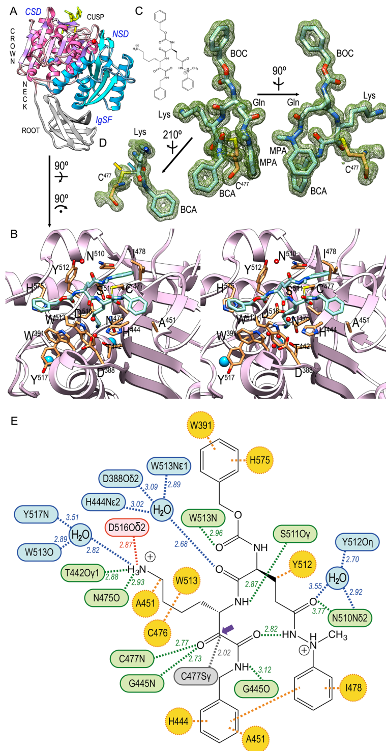
Figure 2. Interactions of the Kgp-KYT-36 complex. (A) Ribbon plot of Kgp, which mimics a tooth, whose crown encompasses the cusp in the top and consists of the NSD (blue ribbon) and CSD domains (magenta ribbon). Domain IgSF (grey ribbon) features the tooth root. KYT-36 is displayed as yellow sticks for reference. (B) Close-up of the tooth cusp encompassing the active site. The left runs from left (non-primed sub-sites) to right (primed sub-sites). Only the CSD is displayed as a plum ribbon for clarity. Kgp residues relevant for the complex are shown for their side chains (carbons in sandy brown) and labeled. The proposed catalytic triad is C 477 , H 444 and D 388 30 . Solvent molecules and structural sodium cations are depicted as red and blue spheres, respectively. KYT-36 is shown as a stick model with carbons in light blue. (C) Structure of KYT-36 and Kgp catalytic residue C 477 superposed with a (2mF obs -DF calc )-type Fourier map contoured at 0.8σ (left) and after a 90°-rotation (right). The five moieties of the inhibitor (see Fig. 1) are labeled. The inset in the top left depicts the chemical structure of the inhibitor for reference. (D) Detail of (C, left) after reorientation depicting the pseudo-covalent bond (2.02 Å) between C 477 S γ (yellow arrow) and the carbonyl carbon of LYS (blue arrow), which mimics the scissile carbonyl
