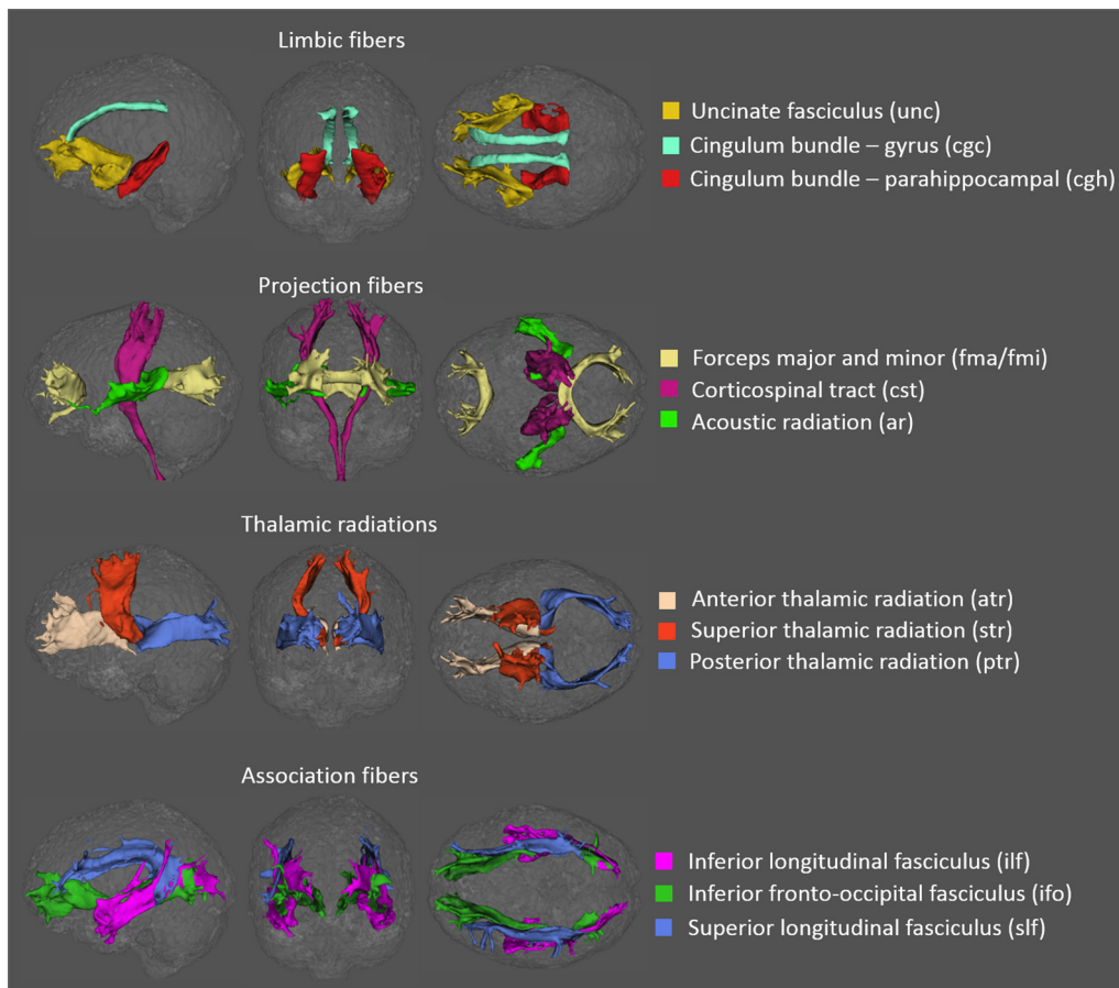
Fig. 1. White matter tracts of interest in one cognitively normal subject generated using probabilistic tractography rendered in sagittal (left), coronal (center), and axial (right) views. The 27 tracts of interest were grouped into five categories: the brainstem (not shown here), limbic fibers connecting the limbic system (first row), projection fibers (second row), thalamic radiations (third row), and association fibers (fourth row).
