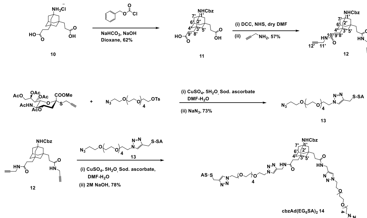
Scheme 3. Synthesis of adamantane core divalent sialoside with \text{EG}_6 spacer.
