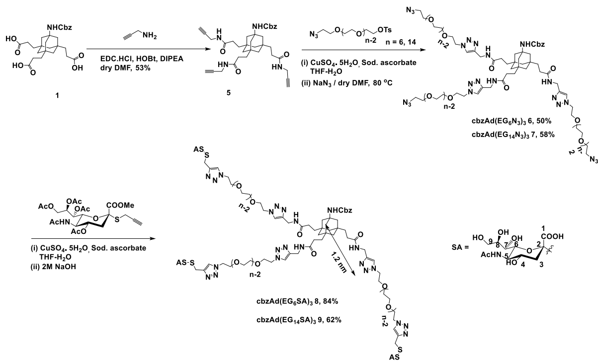
Scheme 2. Synthesis of adamantane core trivalent sialosides with \text{EG}_6 and \text{EG}_{14} spacers.
