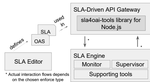
Figure 1: Governify for APIs ' simplified architecture
