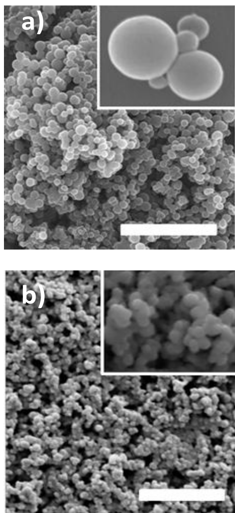
Figure 2. SEM images showing the morphology of Co-CPPs obtained by using different experimental procedures: a) spherical micro-size particles obtained by a diffusion process (bar = 10 \mu\text{m} ) and b) nanoparticles obtained under magnetic stirring (bar = 2 \mu\text{m} ).
