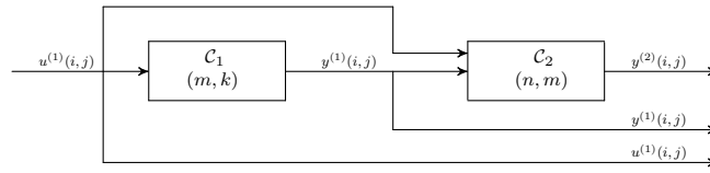
Figure 1. Series concatenation of C_1 and C_2
