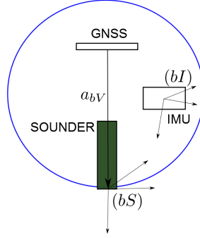
Fig. 3 HydroBall Sketch. The lever-arm vector a_{bV} is defined from the GNSS antenna center of phase to the SBES transducer acoustic center.
