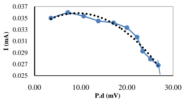
Figure 2. I-V of L.arboreus on ZnO with HgCl 2 .
