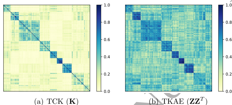
Figure 2: Test set of Jp. Vow. with 80% of missing data. (a) prior \mathbf{K} computed with TCK in input space; (b) dot products \mathbf{Z}\mathbf{Z}^T of the representations in TKAE.
