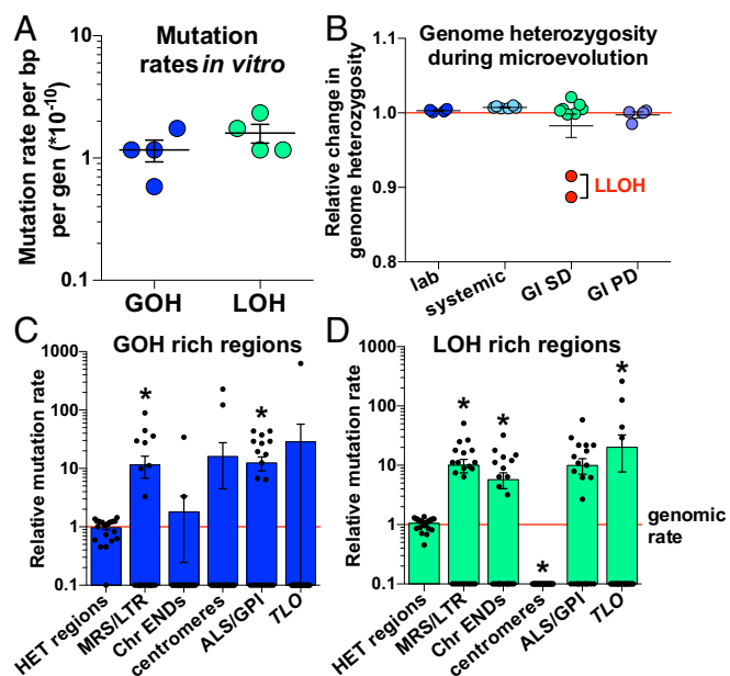
Fig. 3. Mutation rates in C. albicans and the impact of chromosomal features on mutation rates. (A) GOH and LOH mutation rates during in vitro growth. Rates include both SNP and indel events. (B) Fluctuations in genome heterozygosity during microevolution relative to starting heterozygosity levels (red line). Significant decreases in heterozygosity are only observed for two isolates that underwent LLOH events (red symbols). (C and D) GOH (C) and LOH (D) mutation rates in specific regions relative to whole-genome rates. These include heterozygous (HET) regions, repeat regions (MRS and LTR), Chr END regions (final 10 kb of each chromosome arm), centromeres, genes encoding ALS and GPI-linked proteins, and TLO genes. Mutations include both changes in SNPs and indel events. Data points represent independently evolved isolates, and asterisks indicate significant differences relative to whole-genome mutation frequencies ( t test, *P < 0.05 ).
