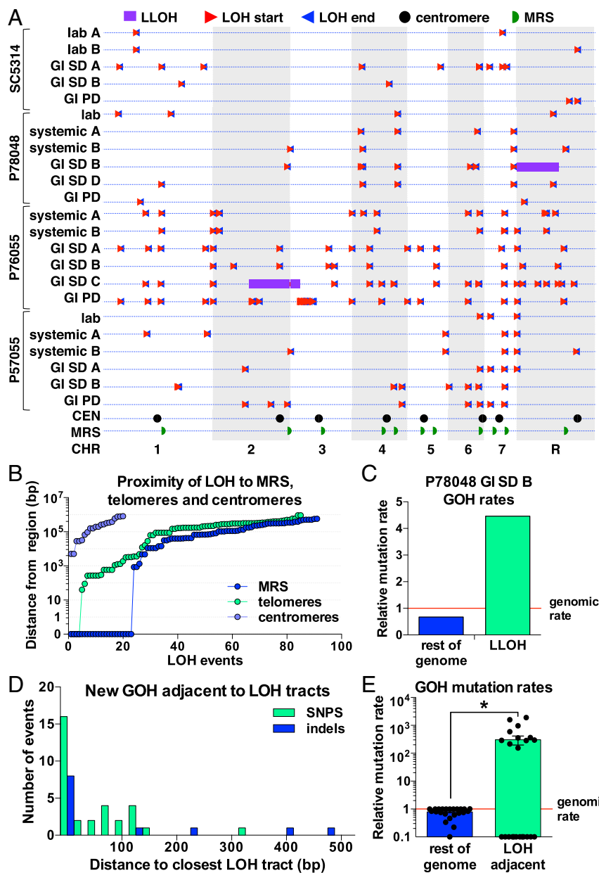
Fig. 5. Relationship between LOH location and different genomic regions. (A) Chromosomal location of all LOH events (using L_{min} ) with triangles marking the start (red) and end (blue) of each event. Location of centromeres (CEN) and MRS regions are shown. (B) Proximity of LOH events to the closest genomic feature, including MRS regions, telomeres (Chr ENDS or TLO genes), and centromeres. Each LOH event is uniquely mapped to the closest of these features on the same chromosome arm. Distances equal to 0 indicate an LOH start site inside the respective genomic region. (C) GOH rates (including SNPs and indels) in the duplicated LLOH region and in the rest of the genome in the P78048 GI SD B isolate, relative to whole genome GOH rates. Only GOH SNPs (base substitutions) were observed in the duplicated LLOH region. (D) Number of GOH events (SNPs and indels per 25 bp) observed within 500 bp of LOH tracts in microevolved isolates. (E) GOH rates (including SNPs and indels) in regions adjacent to LOH tracts (within 500 bp) and in the rest of the genome, relative to whole genome GOH rates. Data points represent independently evolved isolates, asterisks indicate significant differences relative to whole genome mutation frequencies ( t test, * P < 0.05 ).
