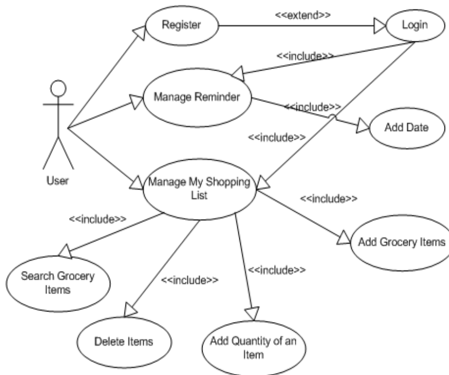
Figure 7. The use case diagram of a mobile app for creating and managing grocery lists.
