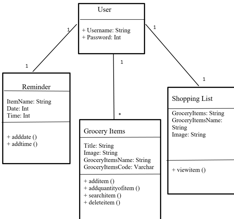
Figure 9. The class diagram of a mobile app for creating and managing grocery lists.
