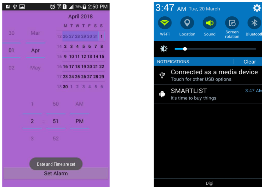
Figure 12. The interface for setting a reminder (left) and the triggered reminder (right).
