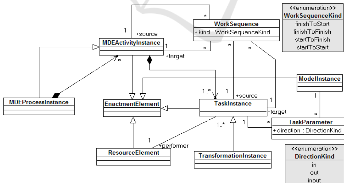
Figure 3: Enactable Process Metamodel.
