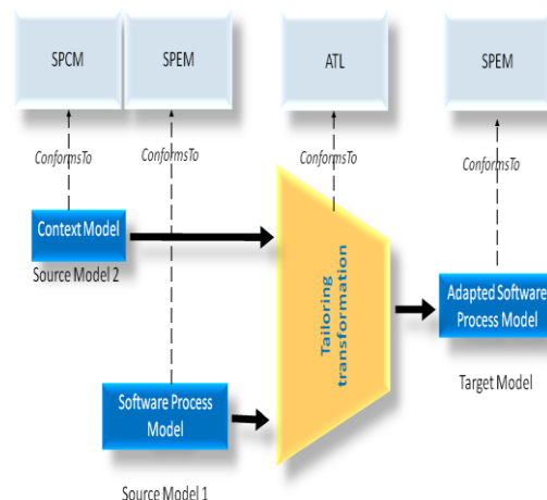
Figure 9: An MDE approach to tailoring (Hurtado and al., 20014).
