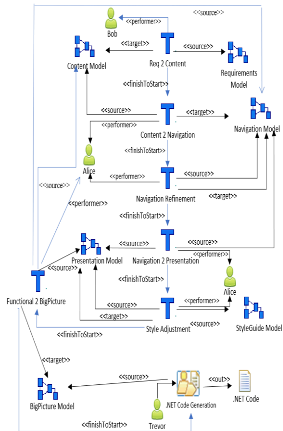
Figure 7: Enactable UWE Process Model.
