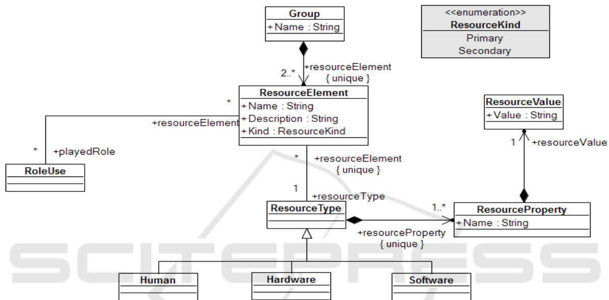
Figure 2: Project Resources Metamodel – PRM.
