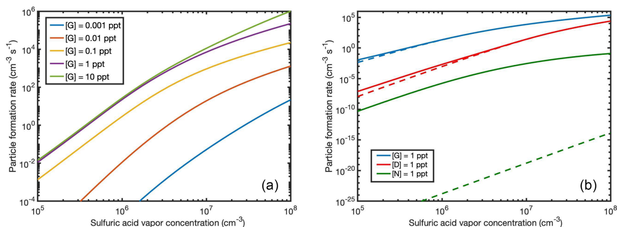
Figure 10. Particle formation rates from sulfuric acid and guanidine at [\text{guanidine}] = 0.001\text{--}10 ppt v in the presence of ions (a), and ion-mediated (solid line) and neutral (dashed line) particle formation rates for guanidine, dimethylamine and ammonia at base concentrations of 1 ppt v (b) as a function of sulfuric acid vapor concentration.
