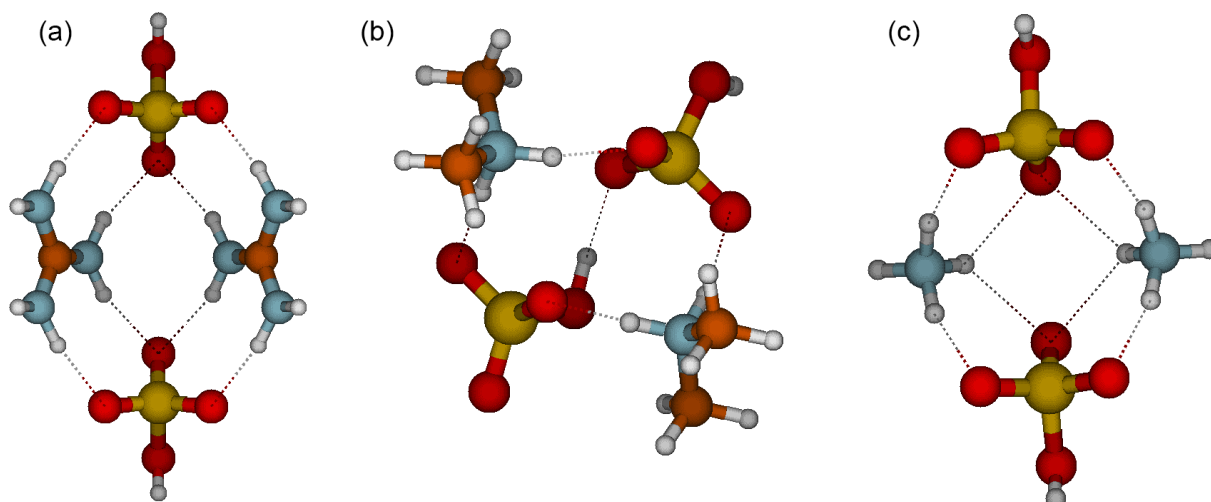
Figure 3. Molecular structures of clusters containing two sulfuric acid and two base molecules for guanidine (a), dimethylamine (b) and ammonia (c). Color coding: brown is carbon, blue is nitrogen, red is oxygen, yellow is sulfur and white is hydrogen.
