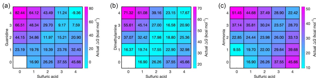
Figure 2. Vapor concentration-dependent Gibbs free energies for electrically neutral acid–base clusters at 298.15 K. Sulfuric acid concentration is 10^7 cm -3 in all cases, and for bases the relative concentrations of [guanidine] = 10^{-5} pptv (a), [dimethylamine] = 1 pptv (b) and [ammonia] = 10^5 pptv (c) are used.
