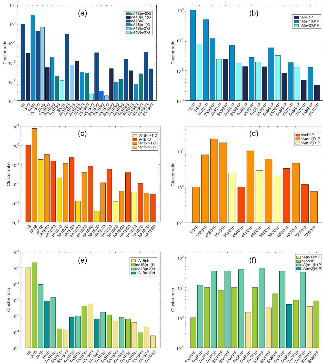
Figure 8. Experimentally determined relative cluster concentrations in negative (a, c, e) and positive (b, d, f) modes for sulfuric acid with guanidine (a, b), dimethylamine (c, d) and ammonia (e, f).
