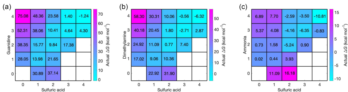
Figure 7. Concentration-dependent Gibbs free energies for protonated-base-containing acid–base clusters at 298.15 K. Sulfuric acid concentration is 10^7 cm -3 in all cases, and for bases the relative concentrations of [guanidine] = 10^{-5} pptv (a), [dimethylamine] = 1 pptv (b) and [ammonia] = 10^5 pptv (c) are used. Note that the x and y axes refer to the numbers of neutral acid and base molecules and each cluster contains one protonated base cation.
