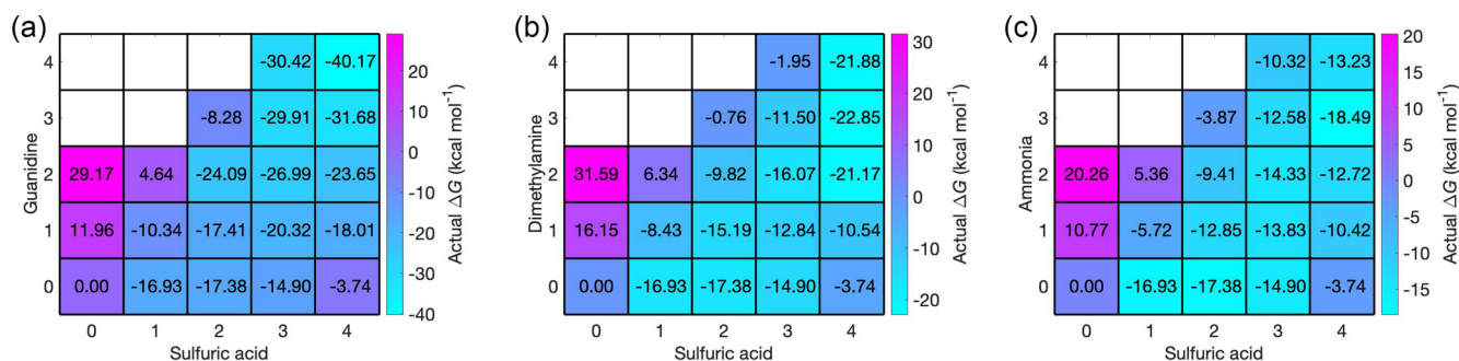
Figure 6. Concentration-dependent Gibbs free energies for bisulfate-containing acid–base clusters at 298.15 K. Sulfuric acid concentration is 10^7 cm -3 in all cases, and for bases the relative concentrations of [guanidine] = 10^{-5} pptv (a), [dimethylamine] = 1 pptv (b) and [ammonia] = 10^5 pptv (c) are used. Note that the x and y axes refer to the numbers of neutral acid and base molecules and each cluster contains one bisulfate anion.
