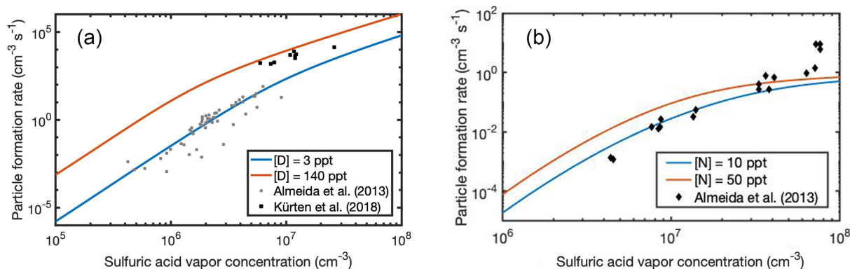
Figure 9. Particle formation rates observed at the CLOUD4 chamber experiment (markers) as a function of sulfuric acid vapor concentration at [D] = 3\text{--}140 ppt v (a) and [N] = 10\text{--}50 ppt v (b), and ACDC simulation results for particle formation in the presence of ions (lines). Note the different scales of x and y axes.
