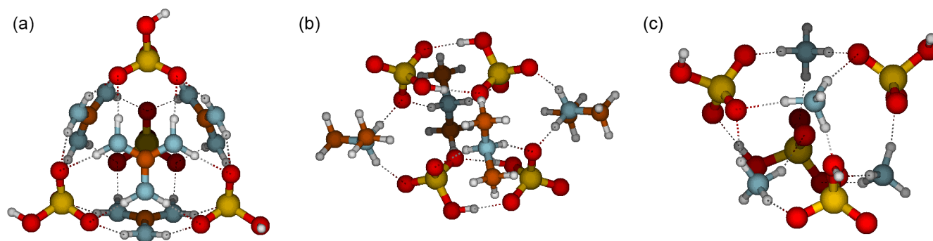
Figure 5. Molecular structures of clusters containing four sulfuric acid and four base molecules for guanidine (a), dimethylamine (b) and ammonia (c). Color coding: brown is carbon, blue is nitrogen, red is oxygen, yellow is sulfur and white is hydrogen.
