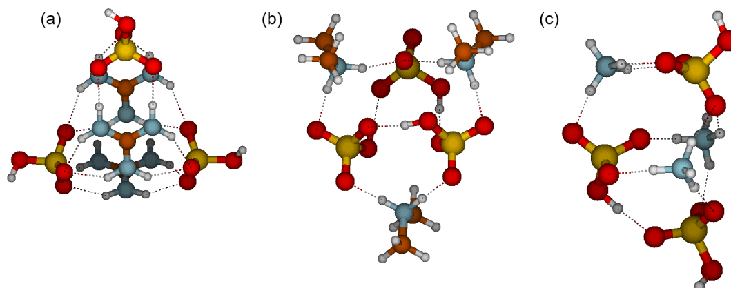
Figure 4. Molecular structures of clusters containing three sulfuric acid and three base molecules for guanidine (a), dimethylamine (b) and ammonia (c). Color coding: brown is carbon, blue is nitrogen, red is oxygen, yellow is sulfur and white is hydrogen.
