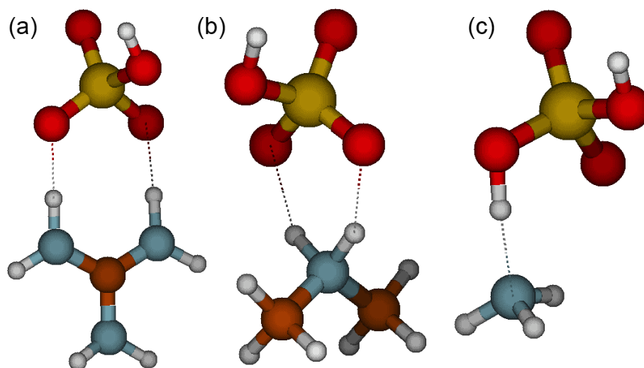
Figure 1. Molecular structures of sulfuric acid heterodimers with guanidine (a), dimethylamine (b) and ammonia (c). Color coding: brown is carbon, blue is nitrogen, red is oxygen, yellow is sulfur and white is hydrogen.
