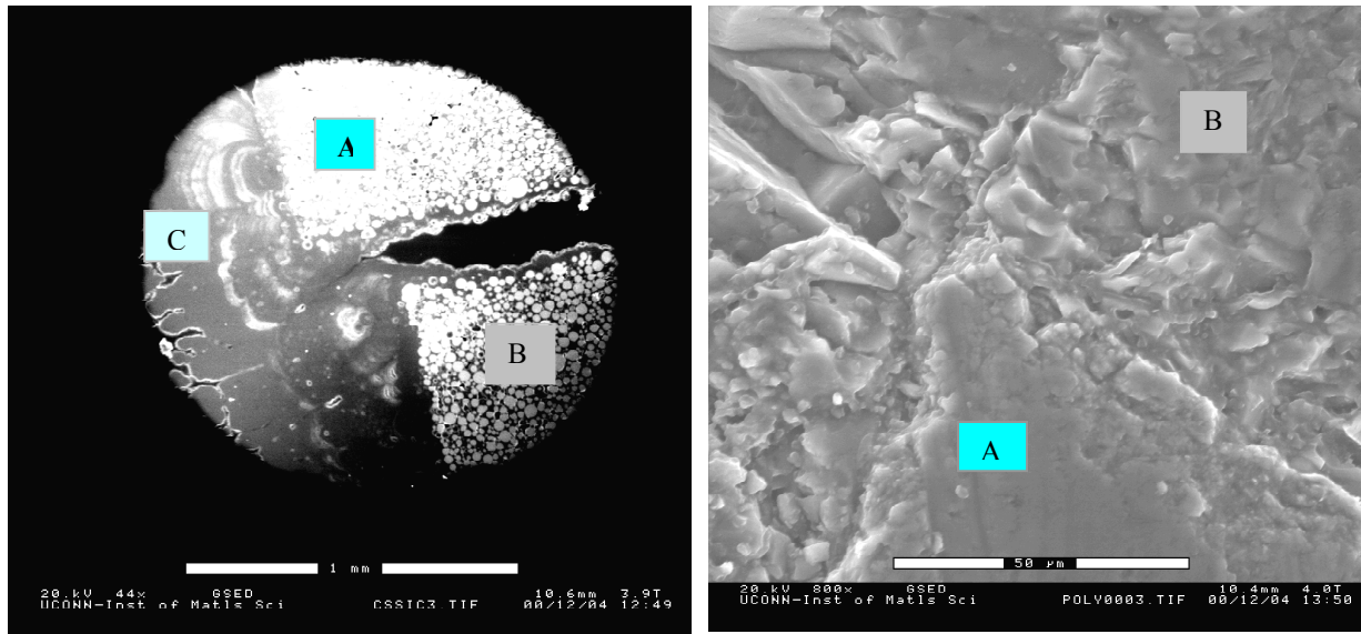
Fig. 7: A cross section of SiC joint over SiC/Mo composite. Fig. 8: Si 3 N 4 deposition over Si 3 N 4 substrate. A, B: Substrate C: Deposit A: Substrate B: Deposit
