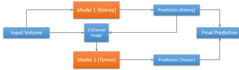
Fig. 1. The processing pipeline composed by two CNNs. First Model computes the prediction for kidney segmentation, which is then used as auxiliary information to the original image to predict the tumor segmentation. Finally, both the predictions of kidney and tumor are joined together to get the final semantic segmentation.
