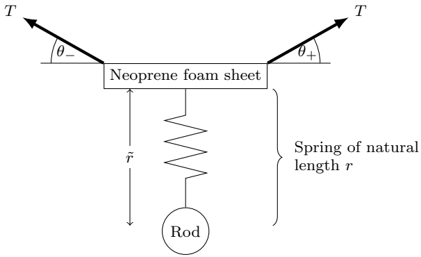
Fig. 5 Model of forces determining the separation between the neoprene foam sheet and a horizontal metal rod. The upper tensions are those applied on this element by neighbouring elements of the sheet. The hook-and-loop fastening that connects the rod to the sheet is modelled as a spring, which is either in tension or compression proportional to its displacement.
