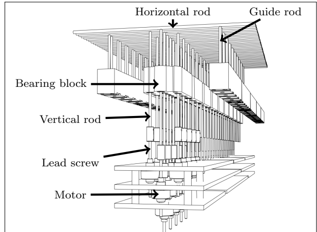
Fig. 3 Perspective drawing of the arrangement of the wave maker linear actuators. The vertical rods are driven up and down, which determines the instantaneous height of each horizontal rod. The neoprene foam sheet of the wave maker is attached to these horizontal rods, so its shape is determined by their heights. The motors are staggered across three horizontal and three vertical planes to enable a tight rod separation of 10 mm.
