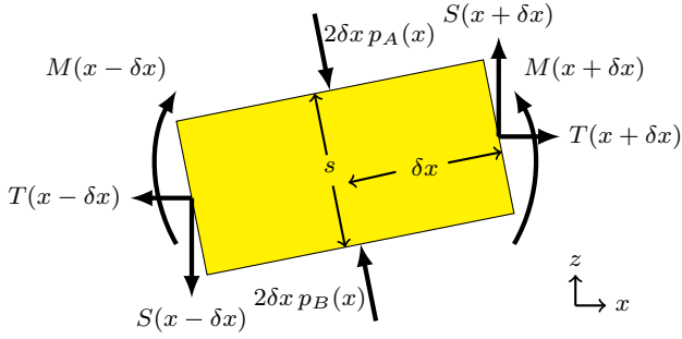
Fig. 4 Forces and moments acting on an element of the sheet (based on Kelly, 2015, p. 202). Shear and tension forces are exerted on each end by the neighbouring elements, in addition to a pair of moments. The fluid above and below the sheet exerts a pressure perpendicular to the sheet.
