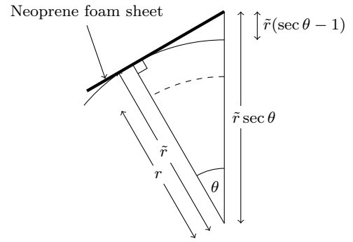
Fig. 6 Variable contact point of the sheet with the rod. For a rod of radius r , the neoprene foam sheet sits at a position given by a larger, variable virtual radius \tilde{r} , due to elasticity in the hook-and-loop attachment. Assuming the bending of the sheet is negligible, its height above the centre of the rod increases by \tilde{r}(\sec \theta - 1) as the contact point moves away from the top in either direction.
