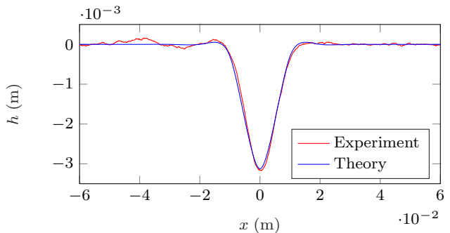
Fig. 10 Comparison of theory with profile recorded on the apparatus for one rod of the wave maker displaced down by 3.81 \times 10^{-3} \text{ m} . The prediction has a small RMS error of 4 \times 10^{-5} \text{ m} and exhibits the small humps around x = \pm 1.3 \times 10^{-2} \text{ m} , which result from the bending stiffness.
