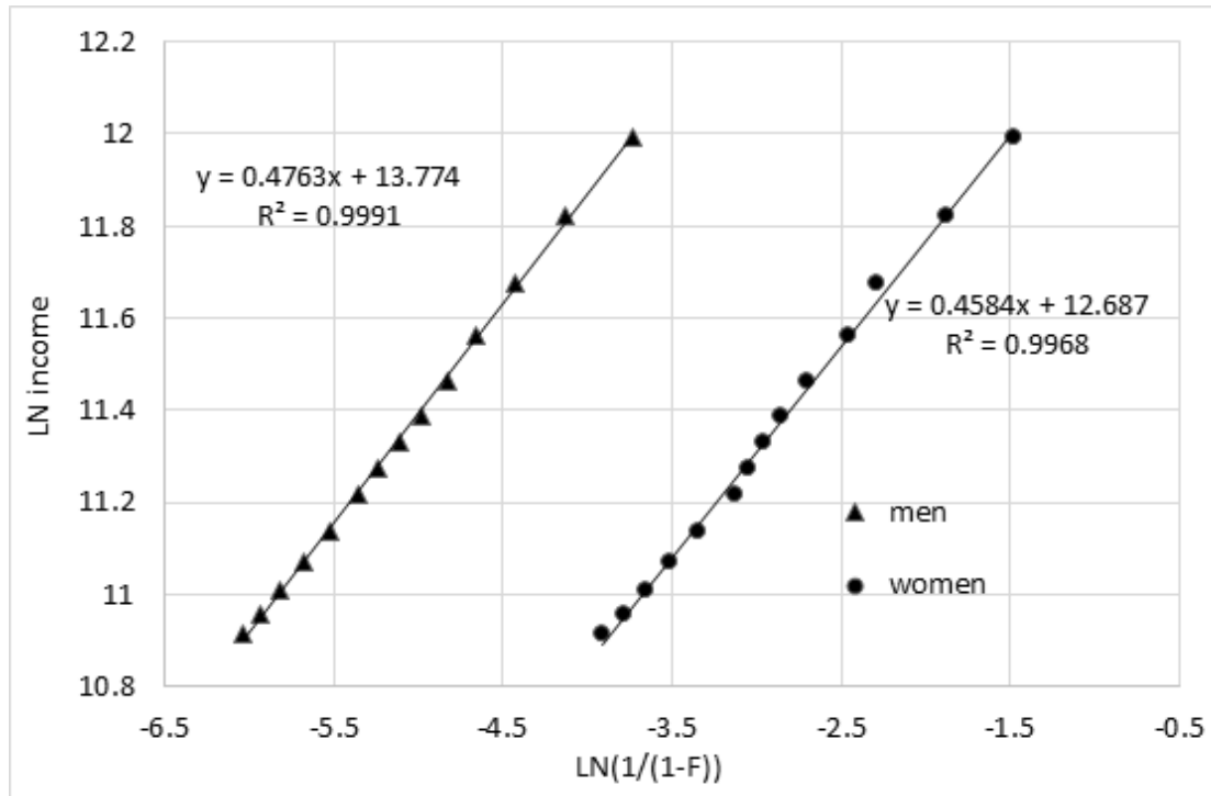
Figure 3a: Pareto curves for the UK - top 1% - 1995
