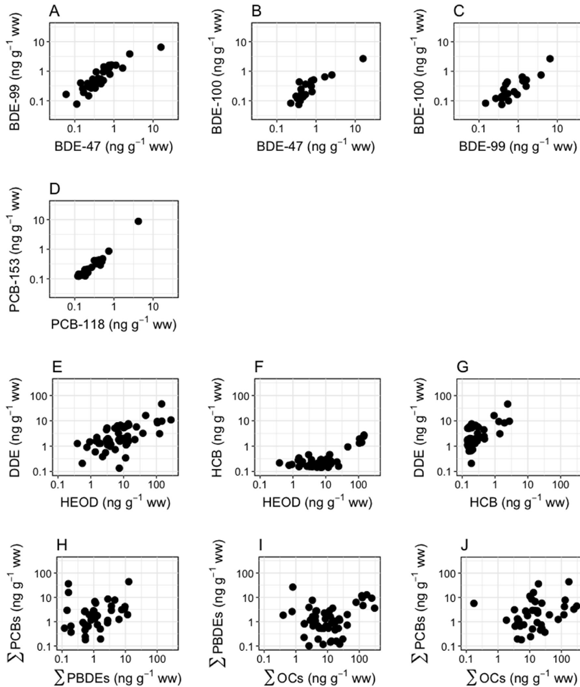
Fig. 6. Relationships between the concentrations of frequently detected ( \geq 30\% of samples) PBDE and PCB congeners, as well as OC compounds. (A–C) Pairwise comparisons of PBDE congeners ( n = 3 ). (D) Pairwise comparisons of PCB congeners ( n = 2 ). (E–G) Pairwise comparisons of OCs ( n = 3 ). (H–J) Pairwise comparisons of \Sigma PBDEs, \Sigma PCBs and \Sigma OCs. Results of statistical analyses are provided in Appendix S5 .
