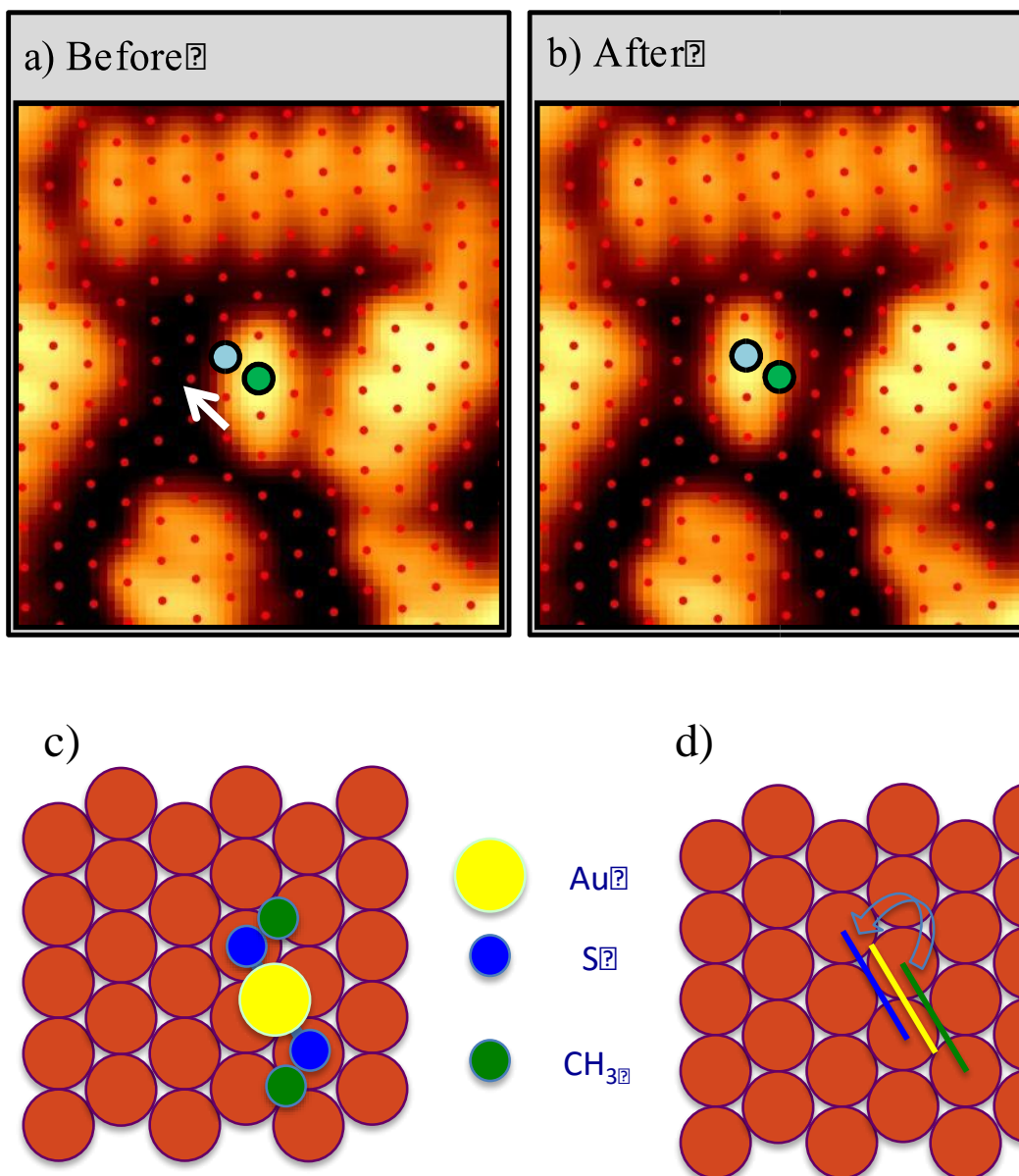
Figure 1. Panels a) and b) show a single \text{Au}(\text{CH}_3\text{S})_2 molecule in two consecutive STM images at 100 K. The initial and final Au-adatom locations are marked in green and blue, respectively. The red dots in both images mark the locations of bridge sites in the underlying Au lattice, deduced from the positions of the \text{Au}(\text{CH}_3\text{S})_2 molecules. Panel c) shows a ball model for a single \text{Au}(\text{CH}_3\text{S})_2 molecule on Au(111). Panel d) illustrates how a single molecule hops between two nearest neighbor adsorption sites via a transition state. The green stick represents the molecule in its initial location and the blue stick represents the molecule in its final location. In the transition state represented by the yellow stick, the Au adatom occupies the bridge site with the S atoms “bridge-bonded” to Au atoms in the substrate. The S atom sits above a bridge site, although it is not clear either this represents a true bridge bond between a S atom and two Au atoms in the substrate.
