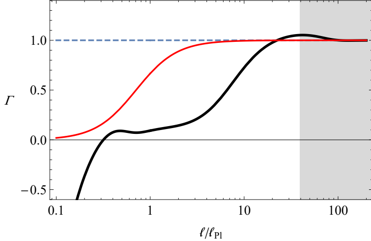
Figure 3. The scaling parameter (4.12) in GFT/spin foams/LQG (solid thick black curve) and theories with monotonic flow from below with d_S^{\text{UV}} = 2 (solid thin red curve), where \ell is a length scale. These curves are obtained from the ad hoc analytic profiles shown in Figs. 1 and 2. The region where discreteness effects become important in GFT/spin foams/LQG (black thick curve plunging down to \Gamma < -3 ) is not shown in the plot. In this figure, the mesoscopic scale \ell_* is around the local maximum at \sim 40 \ell_{\text{Pl}} ; this scale marks the border of the shaded region where 0 < \Gamma_{\text{meso}} - 1 \ll 1 . The dashed line is the IR asymptote.
