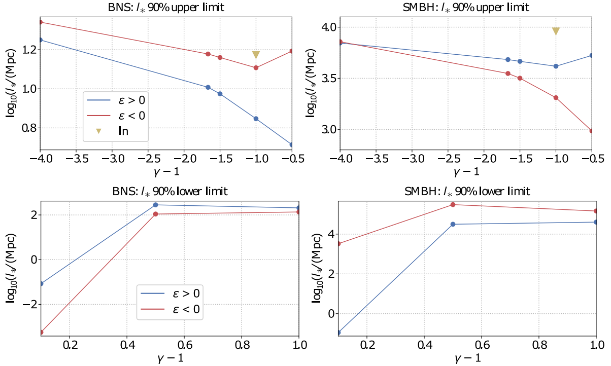
Figure 4. Upper bounds (top plots, for \gamma < 1 ) and lower bounds (bottom plots, for \gamma > 1 ) on \ell_* at the 90% confidence level, for the BNS and SMBH observations, as in Tab. 3. Blue and red show the two cases \epsilon > 0 and \epsilon < 0 in (5.23), while the yellow arrow shows the result for the logarithmic distance relation (5.24).
