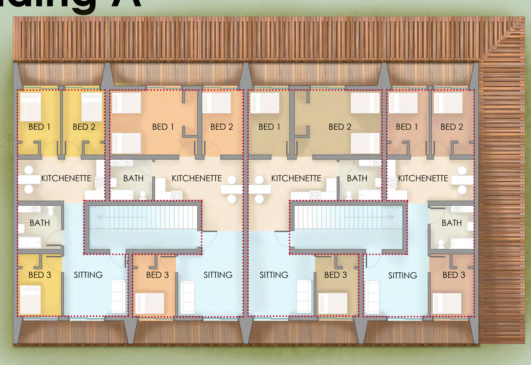
Second Floor Plan Building A
