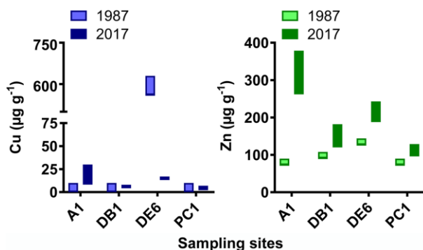
Figure 7. Historical comparison between Fucus sp. samples collected in 1987 and 2017 from Amlwch (site A1), Dulas Bay (site DB1), Dulas Estuary (site DE6) and Porth Cwyfan (site PC1) for Cu and Zn concentration. Boxes show minimum and maximum concentration ranges.
