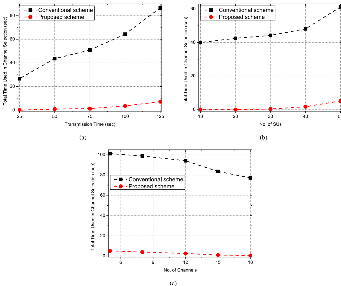
FIGURE 12. Time consumed for channel selection in the proposed vs. the conventional scheme. (a) Time consumed in channel selection under varying transmission times. (b) Time consumed in channel selection under varying number of SUs. (c) Time consumed in channel selection under varying number of licensed channels.
