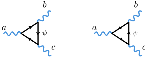
Fig. 1.4. Anomalous triangle diagrams. The fermion loop is reversed on the right.
