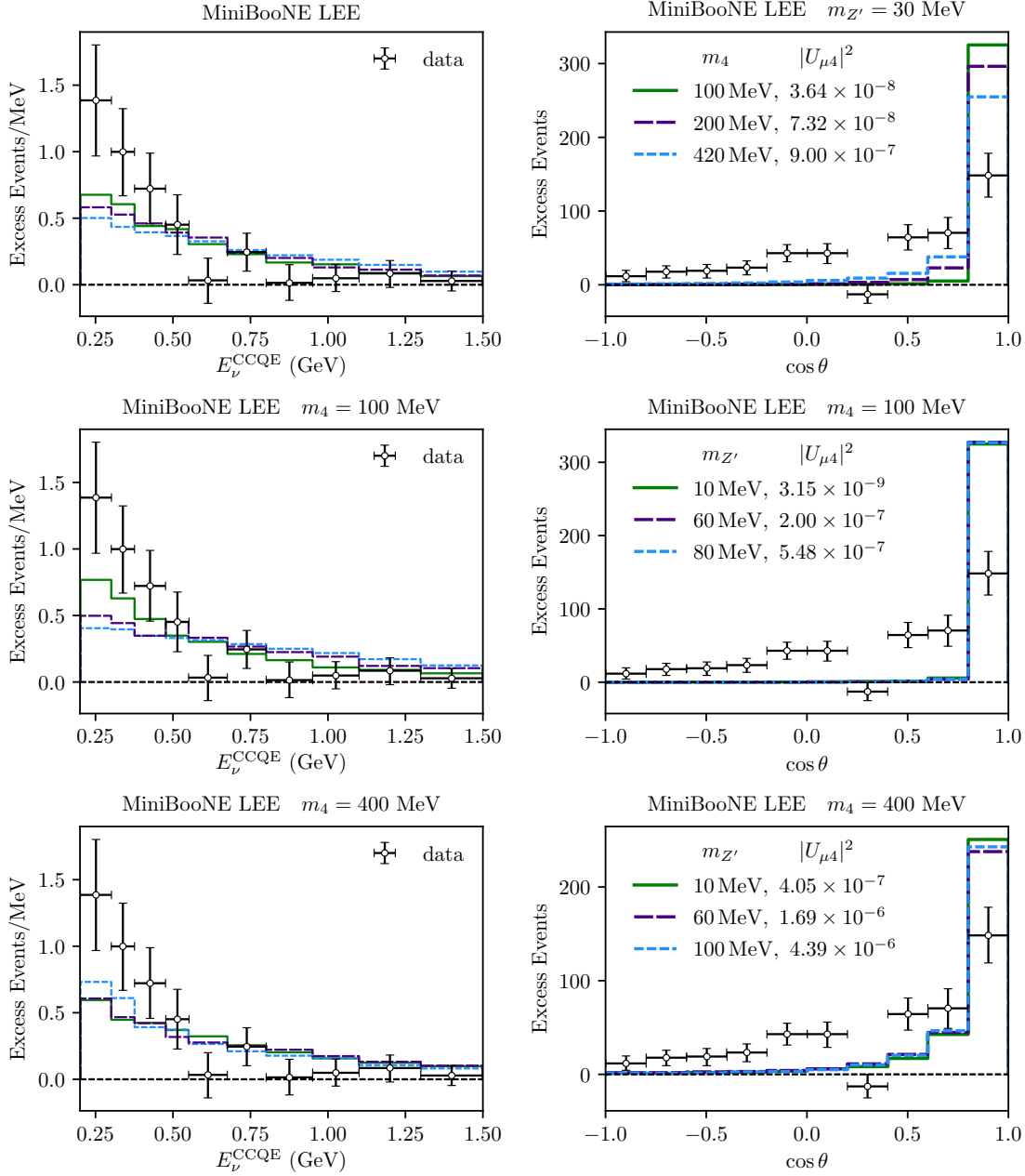
Fig. 6.4. Data and new physics prediction for the reconstructed neutrino energy at MiniBooNE under the assumption of CCQE scattering ( left ), and for the cosine of the angle between the visible EM and the neutrino beam ( right ). We fix couplings so that the total number of events at MiniBooNE equals 334.
