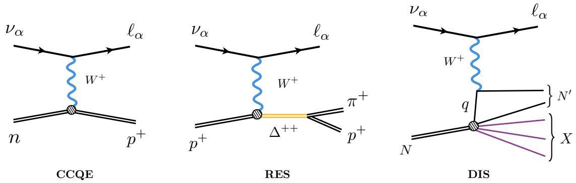
Fig. 2.6. The CC neutrino-nucleon scattering relevant for GeV neutrinos. From left to right, the CC quasi-elastic (CCQE), resonant (RES) and deep-inelastic scattering (DIS) regimes. Analogous diagrams exist for NC scattering.
