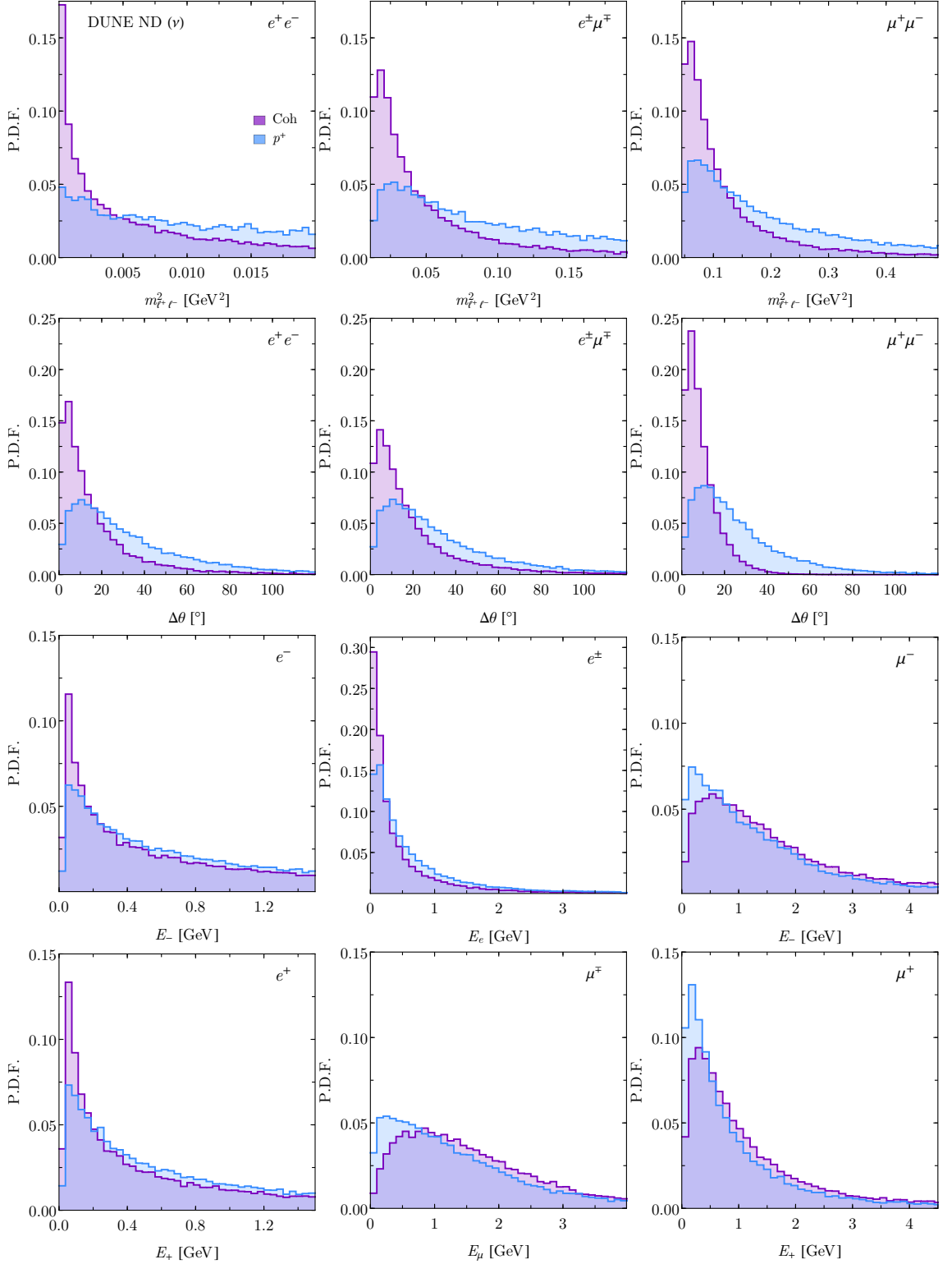
Fig. C.1. Flux convolved neutrino trident production distributions for DUNE ND in neutrino mode. In purple we show the coherent contribution in ^{40}\text{Ar} and in blue the incoherent contribution from protons as targets only (including Pauli blocking). The coherent and incoherent distributions are normalized independently. The relative importance of each contribution as a function of E_\nu can be seen in Fig. 3.6.
