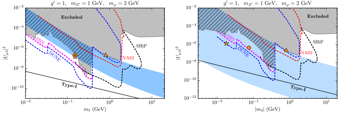
Fig. 5.3. The region of interest for neutrino mass generation in our model in the parameter space of the \nu_5 (left) and \nu_4 (right) mass states. We require m_3 = \sqrt{\Delta m_{\text{atm}}^2} and vary 1\% < m_4/m_5 < 99\% . Our BPs are \triangle ) m_5 = 800 MeV, m_4/m_5 = 99\% , \circ ) m_5 = 150 MeV, m_4/m_5 = 50\% and \star ) m_5 = 150 MeV, m_4/m_5 = 12\% . All bounds and projections displayed assume \chi = \lambda = 0 . The dashed black line shows the equivalent Type-I seesaw contribution to the light neutrino mass.
