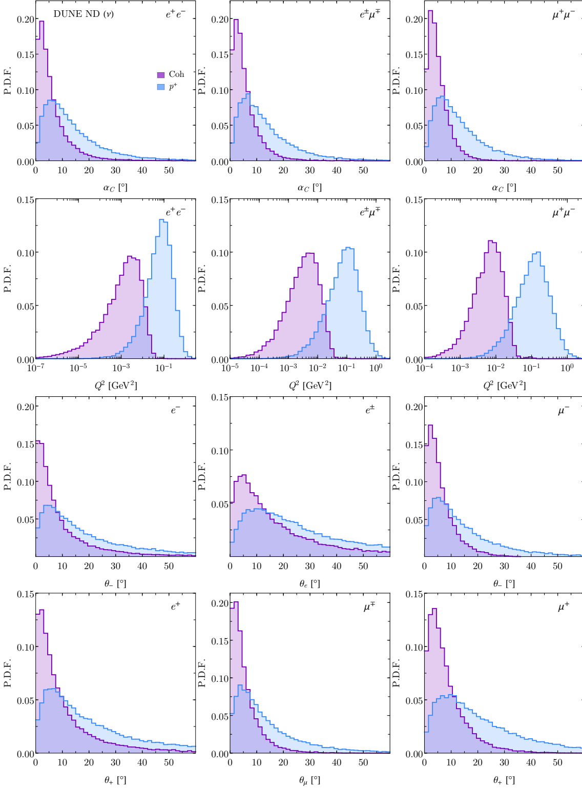
Fig. C.2. Flux convolved neutrino trident production distributions for DUNE ND in neutrino mode in additional variables. In purple we show the coherent contribution in ^{40}\text{Ar} and in blue the incoherent contribution from protons as targets only (including Pauli blocking). The coherent and incoherent distributions are normalized independently.
