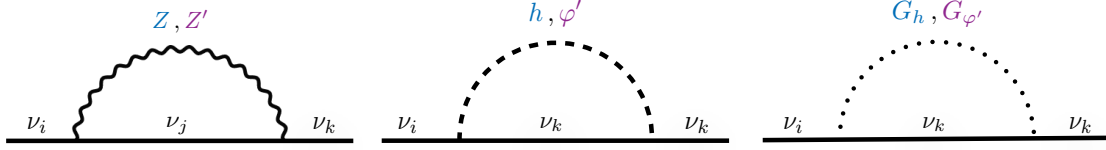
Fig. 5.2. The three contributions to the neutrino self-energy arising from novel bosons in the theory.
