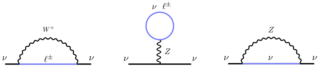
Fig. 2.5. Finite temperature and density corrections to the neutrino self-energy. These can be used to infer the effective matter potential for neutrinos.
