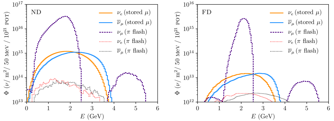
Fig. 7.2. The neutrino flux at the near (left) and far (right) detectors of \nu STORM. Note that the neutrinos from stored muons are separated from the ones generated in the pion flash through timing.
