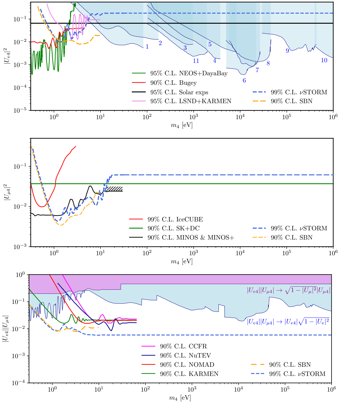
Fig. 7.5. Laboratory bounds on the active-heavy mixing for the 3+1 model with m_4 \approx \Delta m_{41}^2 . Constraints on mixing with electron flavour (top), muon flavour (middle), and the product of the two (bottom) are shown. The numbered bounds on |U_{e4}| come from kink searches in \beta -decay and are all at 95% C.L., except 2 and 9, which are at 90% C.L. The projected sensitivities for SBN [403] and \nu STORM shown as orange and blue dashed lines, respectively.
