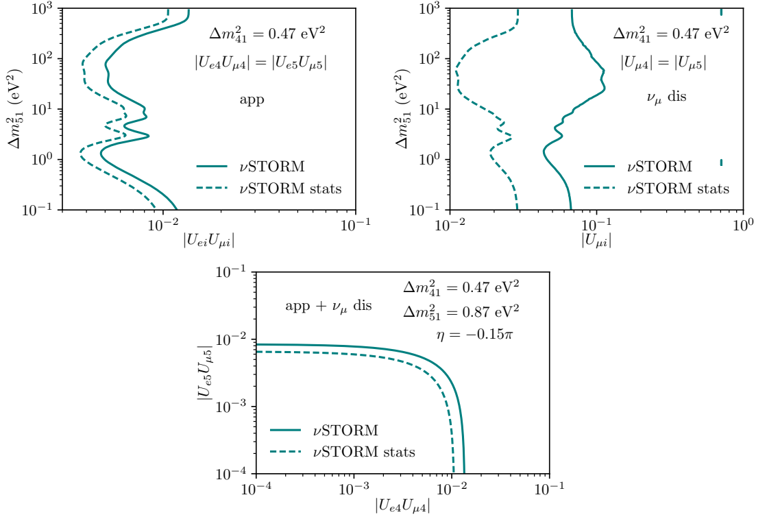
Fig. 7.6. The sensitivity of \nu STORM to short-baseline oscillations in a 3+2 model at 99% C.L. Top left shows the result of an appearance experiment, top right of a muon-disappearance experiment, and bottom of both channels combined.
