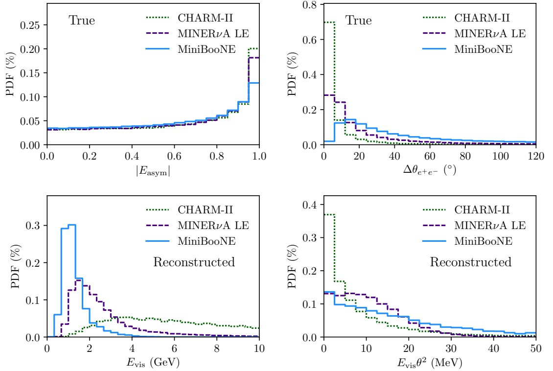
Fig. 6.5. Kinematical distributions for the new physics events at CHARM-II, MINER \nu A LE and MiniBooNE for the BP. We show the energy asymmetry ( top left ), the electron separation angles ( top right ), both at MC truth level. We also show reconstructed (after smearing) total visible energy E_{\text{vis}} ( bottom left ) and E_{\text{vis}}\theta^2 ( bottom right ).
