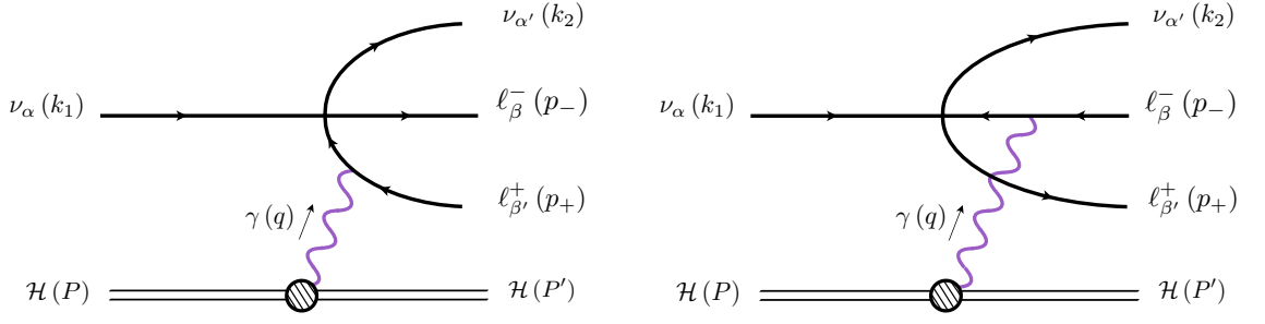
Fig. 3.1. Diagrams contributing to the neutrino trident process in the four-point interaction limit of the Standard Model.
