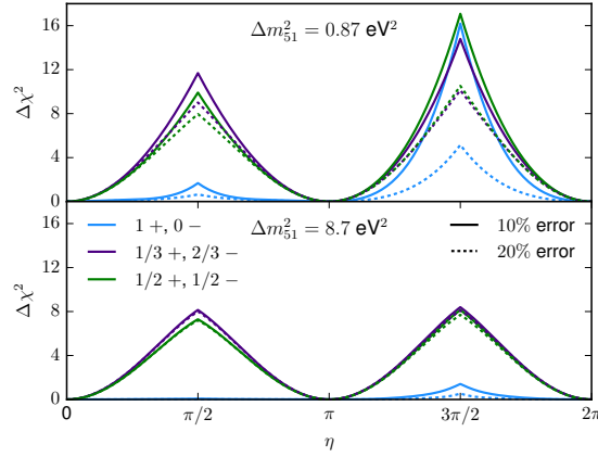
Fig. 7.7. The sensitivity of \nu STORM to the CP violating phase \eta when giving all other parameters 10% and 20% gaussian priors. The top axes show the choice of \Delta m_{51}^2 = 0.87 \text{ eV}^2 , while the bottom axes show a ten times larger value. We use three different configurations: 100% \mu^+ runtime, 66% \mu^- and 33% \mu^+ runtime, and 50% runtime each. The other parameters in the 3+2 model are assumed to be \Delta m_{41}^2 = 0.47 \text{ eV}^2 , |U_{e4}| = 0.13 , |U_{e5}| = 0.14 , |U_{\mu 4}| = 0.15 and |U_{\mu 5}| = 0.13 .
