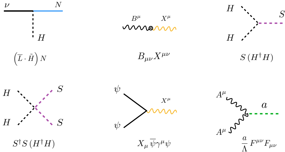
Fig. 1.3. Diagrammatic representation of all portal couplings discussed here. From left to right, the top row shows the neutrino, vector and d = 4 Higgs portal. The bottom row shows the super-renormalizable d = 3 Higgs portal, the fermionic portal and the non-renormalizable pseudo-scalar portal.
