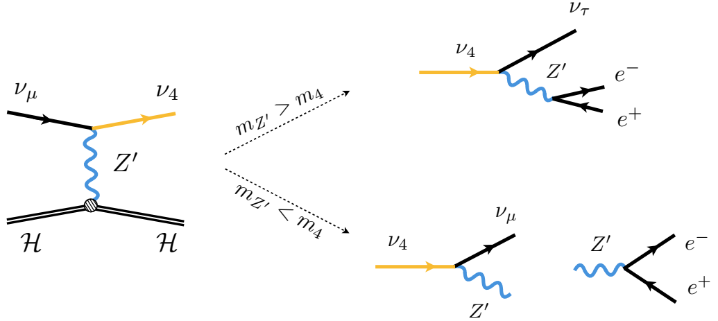
Fig. 6.1. The dark neutrino signal at MiniBooNE. We show the two phenomenological realisations of the dark neutrino model with a heavy (top) and light (bottom) mediator. In the heavy case, large |U_{\tau 4}|^2 is required to shorten the \nu_4 lifetime.
