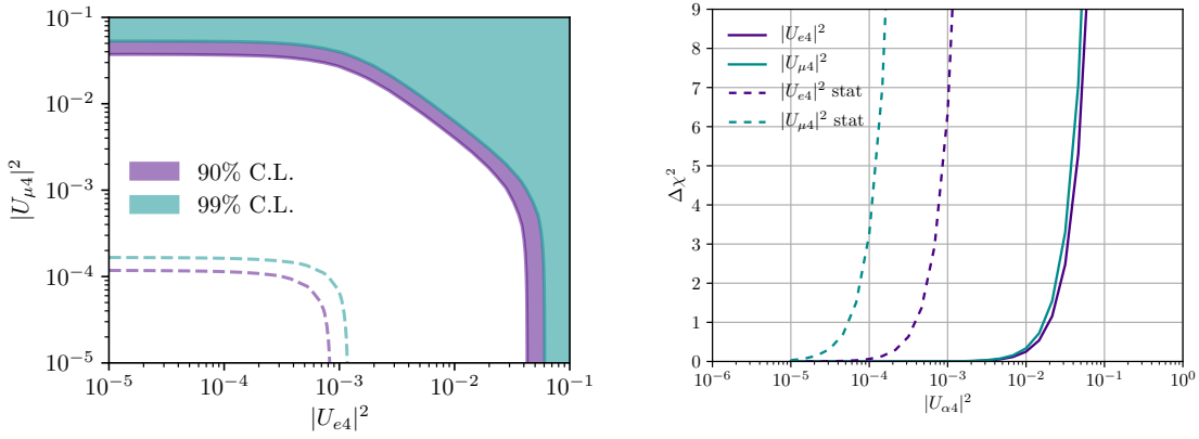
Fig. 7.9. Sensitivity to non-unitarity in the integrated-out sterile case. Dashed lines stand for the statistical limit at \nu STORM.
