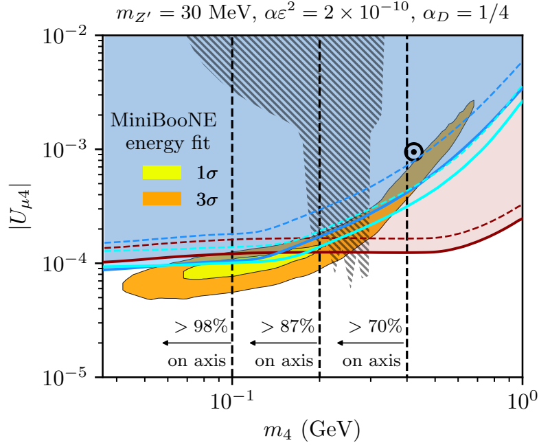
Fig. 6.7. The fit to the MiniBooNE energy distribution from [148] is shown as closed yellow (orange) region for one (three) sigma C.L., together with the benchmark point ( \odot ). Our constraints are shown at 90% C.L. for MINER \nu A LE in blue (solid – 30% background normalization uncertainty, dashed – conservative 100% case), for MINER \nu A ME in cyan (solid – 40% background normalization uncertainty, dashed – conservative 100% case), and for CHARM-II in red (solid – 3% background normalization from the sideband constraint, dashed – conservative 10% case). Vertical lines show the percentage of excess events at MiniBooNE that lie in the most forward angular bin. Exclusion from heavy neutrino searches is shown as a hatched background. Other relevant assumed parameters are shown above the plot; changing them does not alter our conclusion.
