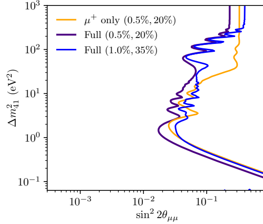
Fig. 7.4. Variations of the \nu_\mu disappearance sensitivity at 99% C.L.. In purple, we show the main curve from Fig. 7.3 and in blue we increase all flux related systematic uncertainties to 1% and cross sections \times efficiencies uncertainties to 35%. With the standard systematics, in orange we use only the events from stored muons (larger decay length).
