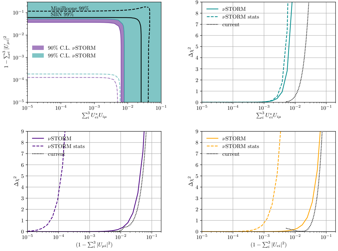
Fig. 7.8. Bounds on the non-unitarity of the mixing matrix in the averaged-out sterile case. Top left shows the two dimensional plane to which \nu_\mu disappearance and \nu_e \rightarrow \nu_\mu appearance experiments are sensitive to. We then show the one-dimensional \Delta\chi^2 profile for appearance (top right), \nu_\mu disappearance (bottom left) and \nu_e disappearance (bottom right). All colorful dashed lines stand for the statistical limit at \nu STORM.
