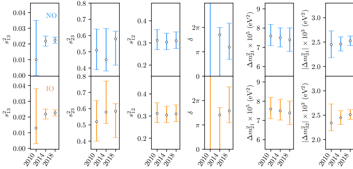
Fig. 2.3. The neutrino oscillation global-fit results in 2010 [77], 2014 [78] and 2018 [79]. We show the best-fit point, together with the 3\sigma regions for normal ordering (NO) and inverted ordering (IO).
