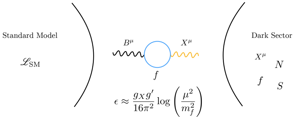
Fig. 1.2. A possibility for a portal between the Standard Model and a dark sector. Fermions f charged under both the hypercharge group and a new U(1) group generate kinetic mixing at loop level between B^\mu and the new boson X^\mu . In the approximate formula for \epsilon , \mu^2 stands for the renormalization scale and g_X to the gauge coupling of the new U(1) .
