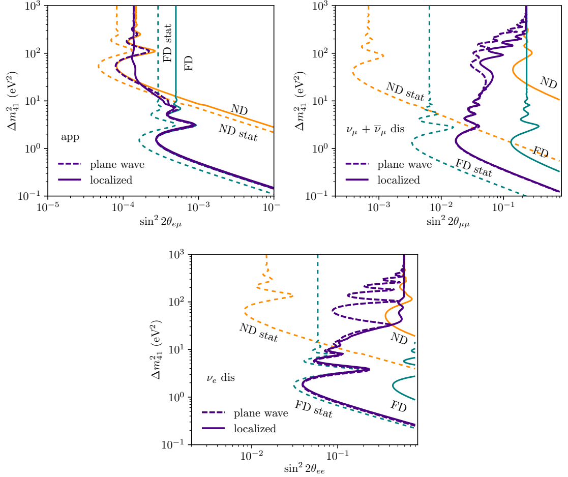
Fig. 7.3. The 99% C.L. sensitivities of \nu STORM to the phenomenological parameters \theta_{e\mu} (top left), \theta_{\mu\mu} (top right), and \theta_{ee} (bottom). The orange (cyan) curves assume only a single near (far) detector, respectively, and do not take localization into account. For those, dashed lines are the statistical limit. The dashed purple curves assume the presence of both detectors. Solid purple curves take localization into account.
