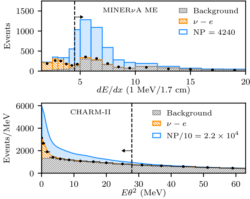
Fig. 6.6. Neutrino-electron scattering data in dE/dx at MINERνA (top) and in E\theta^2 at CHARM-II (bottom). Error bars are too small to be seen. For both experiments, we show the \nu - e signal and total background prediction quoted (after tuning at MINERνA), as well as the NP prediction (divided by 10 at CHARM-II). The cuts in our analysis are shown as vertical lines.
