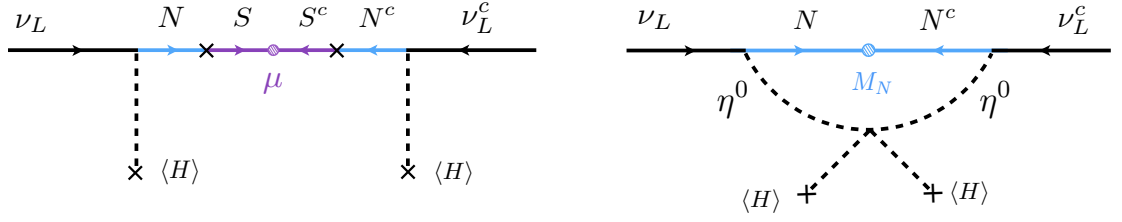
Fig. 2.2. On the left, the inverse seesaw flavour diagram for Majorana neutrino masses. On the right, the flavour diagram for the scotogenic mode. Arrows represent lepton number.
