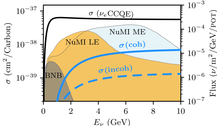
Fig. 6.2. The quasi-elastic cross section on Carbon ( 6p^+ ) is shown as a function of the neutrino energy (solid black line). The coherent (solid blue) and incoherent (dashed blue) scattering NP cross sections are also shown for the benchmark point of [148]. In the background, we show the BNB flux of \nu_\mu at MiniBooNE (light gray), and the NuMI beam neutrino flux at MINER \nu A for the LE (light golden) and ME (light blue) runs in neutrino mode.
