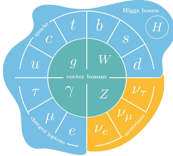
Fig. 1.1. Artistic rendering of the particles in the Standard Model.
