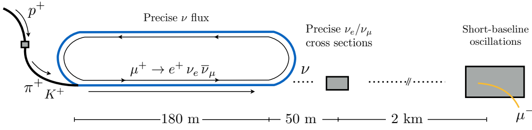
Fig. 7.1. \nu STORM in a diagram.
