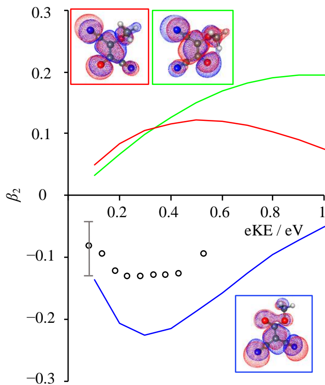
Figure 57 Plot of the experimental (circles) and computed (solid lines) \beta_2 parameters as a function of eKE for the direct detachment channel of the three isomers of the ESI product. The lowest energy isomer, MDCA - , is shown in blue, while the cis- and trans-isomers are shown in green and blue respectively. The relevant Dyson orbitals are inset and follow the same colour scheme.
