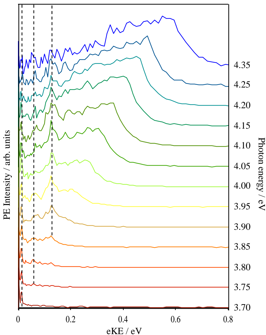
Figure 58 PE spectra of the MDCA - as a function of increasing photon energy. Low energy structured features that remain static in eKE space are highlighted.
