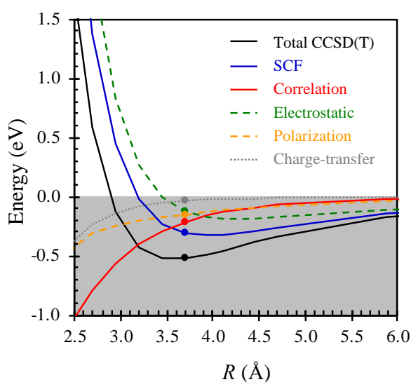
Figure 47 Contributions to the calculated total energy from the SCF and correlation energies. The SCF energy is further decomposed into contributions from electrostatic, polarization and charge-transfer interactions. The points indicate the decomposed energies at the calculated minimum energy geometry. The grey area indicates regions of attractive interactions.
