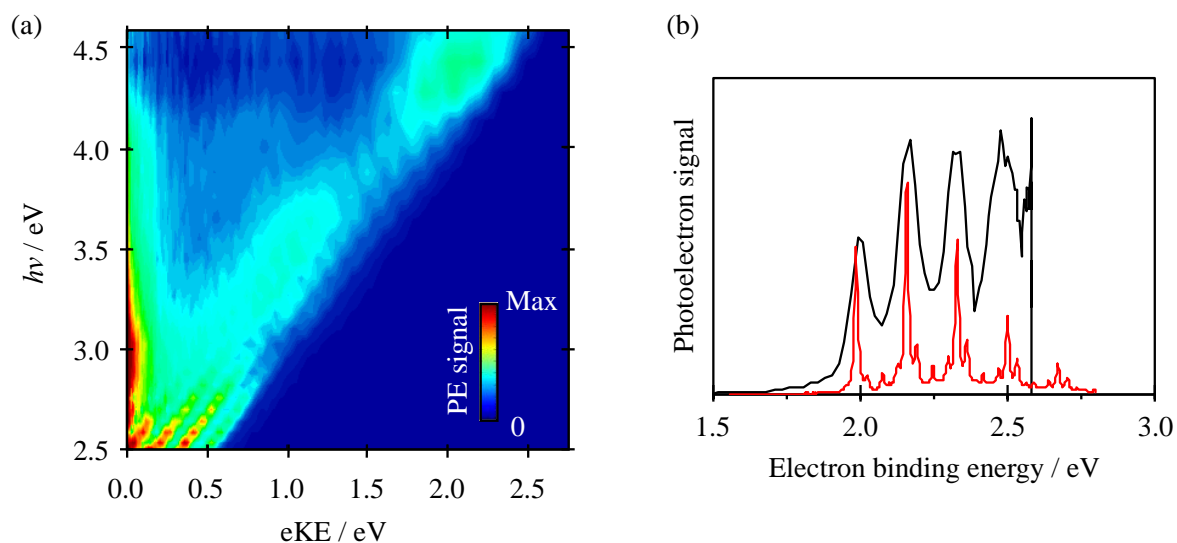
Figure 39 (a) 2D photoelectron spectra of \text{pDNB}^- , where each spectrum has been normalised to its integrated PE signal. (b) Measured (black) and simulated (red) photoelectron spectra (a slice of (a) taken at h\nu = 2.58 \text{ eV} )
