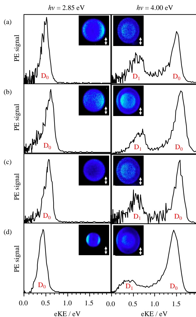
Figure 19 Photoelectron spectra acquired at h\nu = 2.85 and 4.00 eV for (a) \text{Ph}^- , (b) \text{pMPh}^- , (c) \text{pEPh}^- , and (d) \text{pVPh}^- . Respective raw images are inset with the polarization axis of the laser shown by the double arrow. The photoelectron features corresponding to the D_0 and D_1 channels are indicated.
