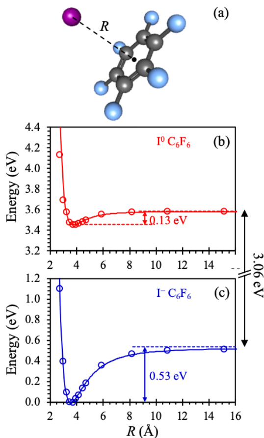
Figure 46 (a) Minimum energy structure of \text{I} \cdot \text{C}_6\text{F}_6 and potential energy curves for (b) \text{I} \cdot \text{C}_6\text{F}_6 and (c) \text{I}^- \cdot \text{C}_6\text{F}_6 as a function of separation between the I and the center of the \text{C}_6\text{F}_6 ring. The solid lines in (b) and (c) are Leonard-Jones potential energy functions with parameters defined in the text.
