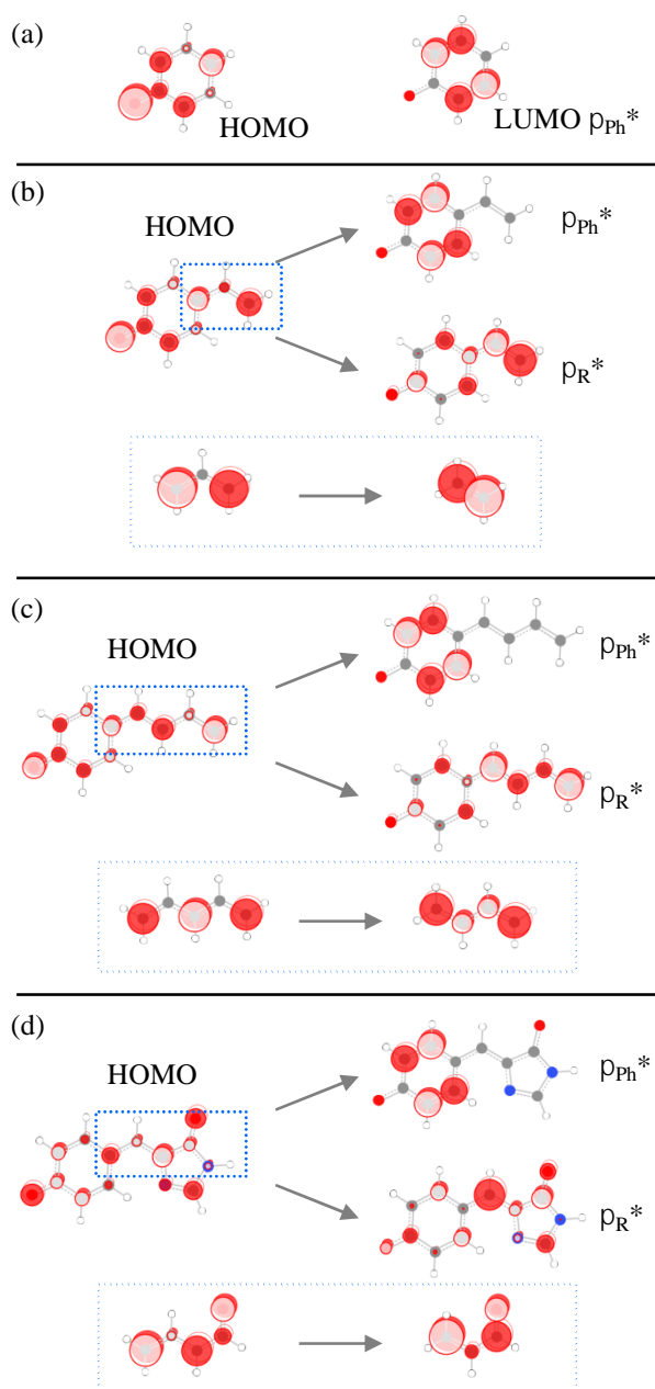
Figure 37 Highest occupied Hückel molecular orbital (HOMO) and lowest unoccupied molecular orbital (LUMO) and \pi_{\text{Ph}}^* and \pi_{\text{R}}^* MOs of (a) \text{Ph}^- , (b) \text{pVPh}^- , (c) \text{pBPh}^- , and (d) \text{HBI}^- . Marked insets in (b) – (d) show the chromophoric MOs involved in the HOMO \rightarrow LUMO transition. It is noted that there is a small contribution of the second unoccupied \pi^* MO of phenolate (b), however this is the same in all molecule, so may be expected to have the same contribution in all anions considered.
