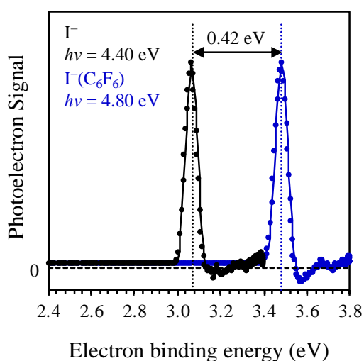
Figure 45 Photoelectron spectra of I^- and I^-\cdot C_6F_6 taken at 4.40 and 4.80 eV, respectively. The vertical dashed lines indicate the peak positions, which are separated by 0.42 eV.
