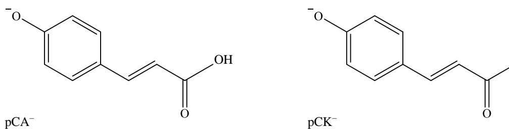
Figure 23 Skeletal representations of two derivatives of the anionic chromophore in PYP, para-coumaric acid ( \text{pCA}^- ) and para-coumaric ketone ( \text{pCK}^- ).
