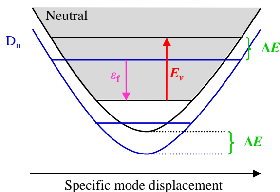
Figure 53 Schematic showing the proposed mechanism for mode facilitated electron loss from an excited state of the anion. The potential energy surface is shown as a blue curve, and that of the neutral ground state as black. The continuum is represented by the shaded grey. The displacement between the two surfaces is equal to the binding energy of the excited state.
