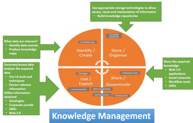
Fig. 3. KM Lifecycle in Learning
