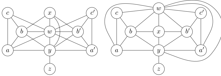
Figure 2: A planar graph from \mathcal{G} with 10 vertices without a 2-PDS partition. On the left, its schematic representation as in Fig. 1; on the right, its planar representation.
