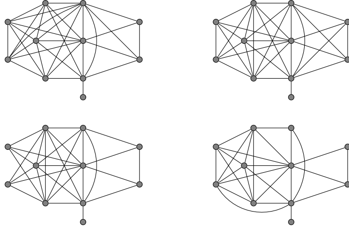
Figure 3: Four graphs with 11 vertices which do not have a 2-PDS partition
