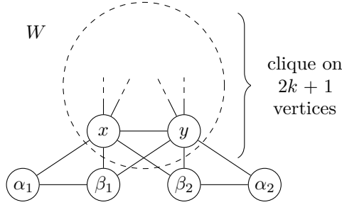
Figure 4: A schematic representation of a graph in \mathcal{H} .
