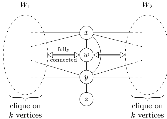
Figure 1: A schematic representation of a graph in \mathcal{G} .
