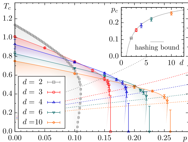
FIG. 3: (Color online) Phase boundaries for different d estimated from Monte Carlo simulations of the respective disordered Potts models representing quantum error correction for d -level quantum systems. The solid lines and shaded areas are guides to the eye. The error threshold p_c(d) corresponds to the point where the corresponding Nishimori lines (dashed) intersects the phase boundaries for different d . This is the maximum disorder rate for which error correction is feasible. Inset: Comparison of the calculated error thresholds for different values of d to the upper bound given by the hashing bound (dotted black line). There is excellent agreement.
