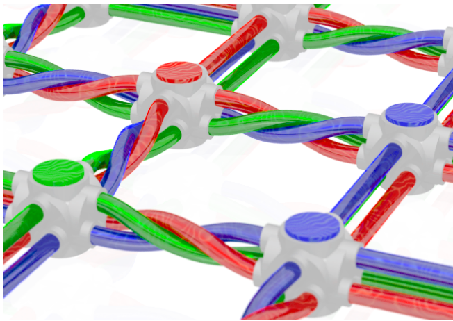
FIG. 2: (Color online) Rendering of the classical three-colored Potts model found in the mapping of an abelian quantum double model with qutrits (i.e., qubits with d = 3 ) on each edge. Quantum errors give rise to disorder in the interactions between neighboring sites, indicated in the form of twisted links. An ordered state in this model (i.e., one predominant color in the system) in spite of these faulty links indicates resilience of the original setup to quantum errors.
