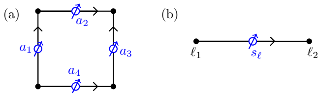
FIG. 1: Numbering and orientation conventions used in the calculations. The quantum spins of the original model are shown as (blue) empty circles on the graph’s edges, whereas the sites of the classical model are shown as (black) solid dots on the vertices. (a) Convention for determining anyon occupancy of a plaquette \square from the quantum spins on the edges. (b) Convention for assigning classical spins S_{\ell_1} and S_{\ell_2} to the vertices and determining the effective \kappa_\ell for a given link \ell .
